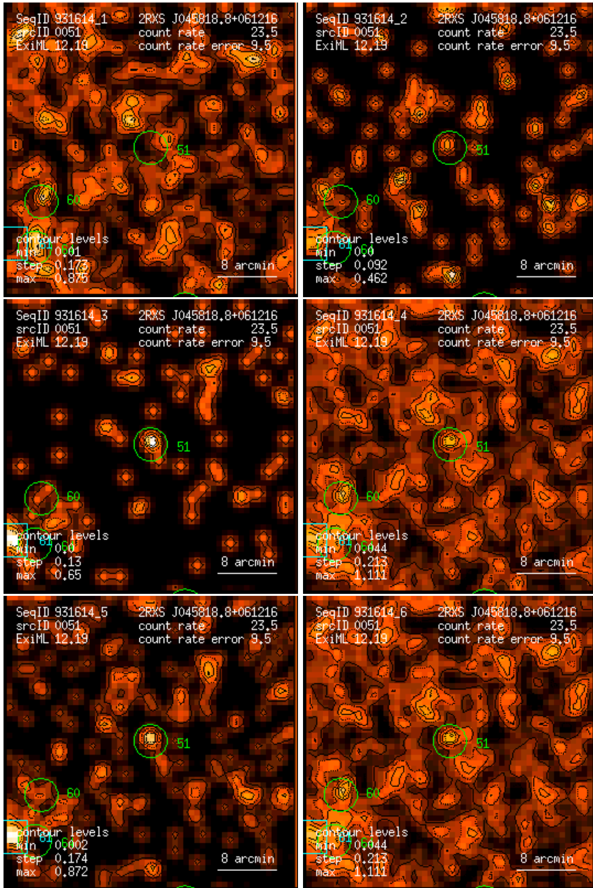
Figure 51: RASS 931614: detection 0051: band rate images, Gaussian filter: (1) PSPC channels 11 – 41, (2) 52 – 90, (3) 91 – 201, (4) 11 – 235, (5) 52 – 201, (6) 11 – 201. Broad band rates in counts/ks. Band rate contour levels in counts/ks/arcmin 2 .
