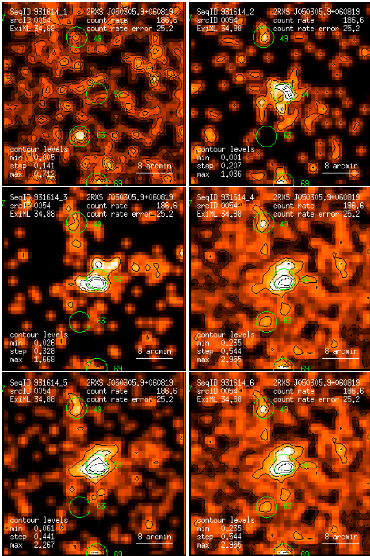
Figure 54: RASS 931614: detection 0054: band rate images, Gaussian filter: (1) PSPC channels 11 – 41, (2) 52 – 90, (3) 91 – 201, (4) 11 – 235, (5) 52 – 201, (6) 11 – 201. Broad band rates in counts/ks. Band rate contour levels in counts/ks/arcmin 2 .
