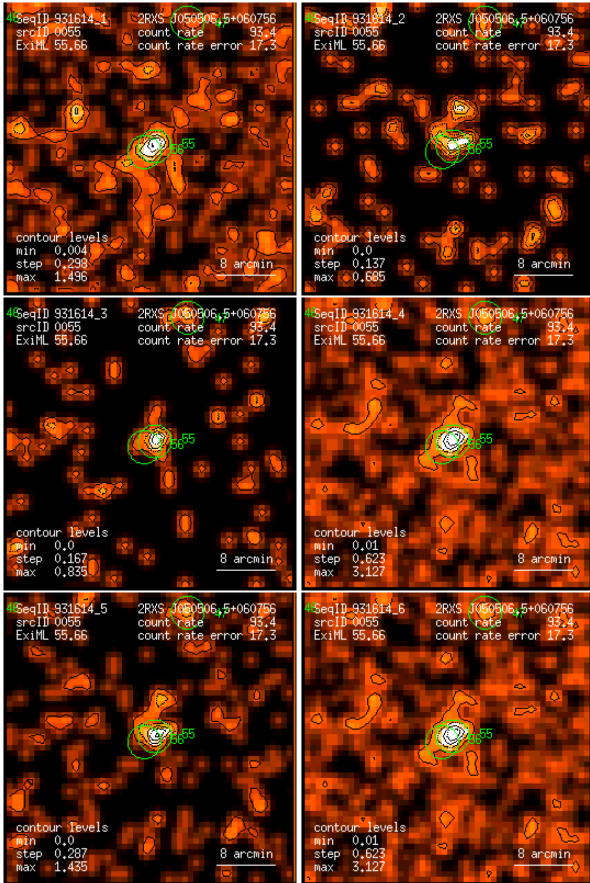
Figure 55: RASS 931614: detection 0055: band rate images, Gaussian filter: (1) PSPC channels 11 – 41, (2) 52 – 90, (3) 91 – 201, (4) 11 – 235, (5) 52 – 201, (6) 11 – 201. Broad band rates in counts/ks. Band rate contour levels in counts/ks/arcmin 2 .
