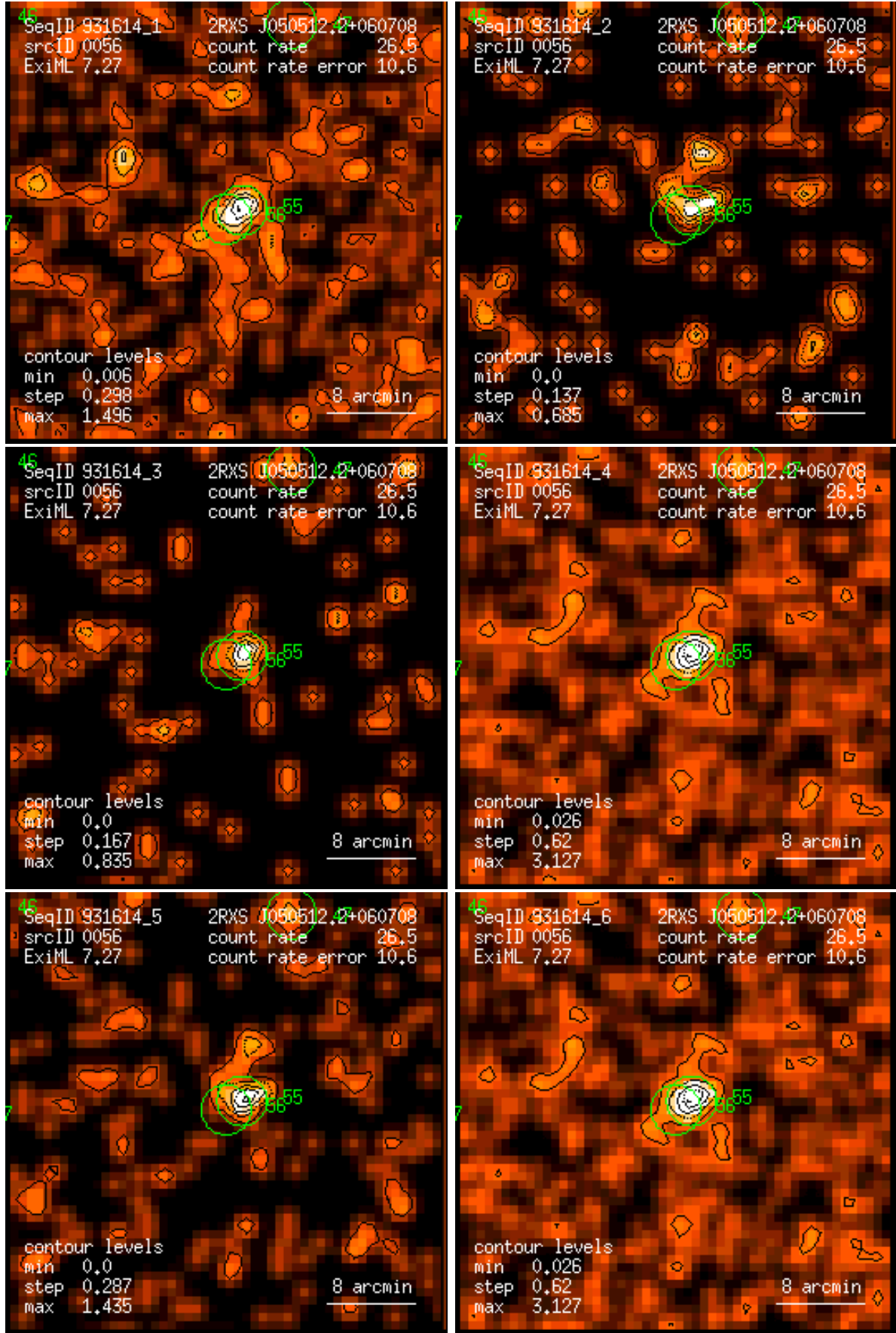
Figure 56: RASS 931614: detection 0056: band rate images, Gaussian filter: (1) PSPC channels 11 – 41, (2) 52 – 90, (3) 91 – 201, (4) 11 – 235, (5) 52 – 201, (6) 11 – 201. Broad band rates in counts/ks. Band rate contour levels in counts/ks/arcmin 2 .
