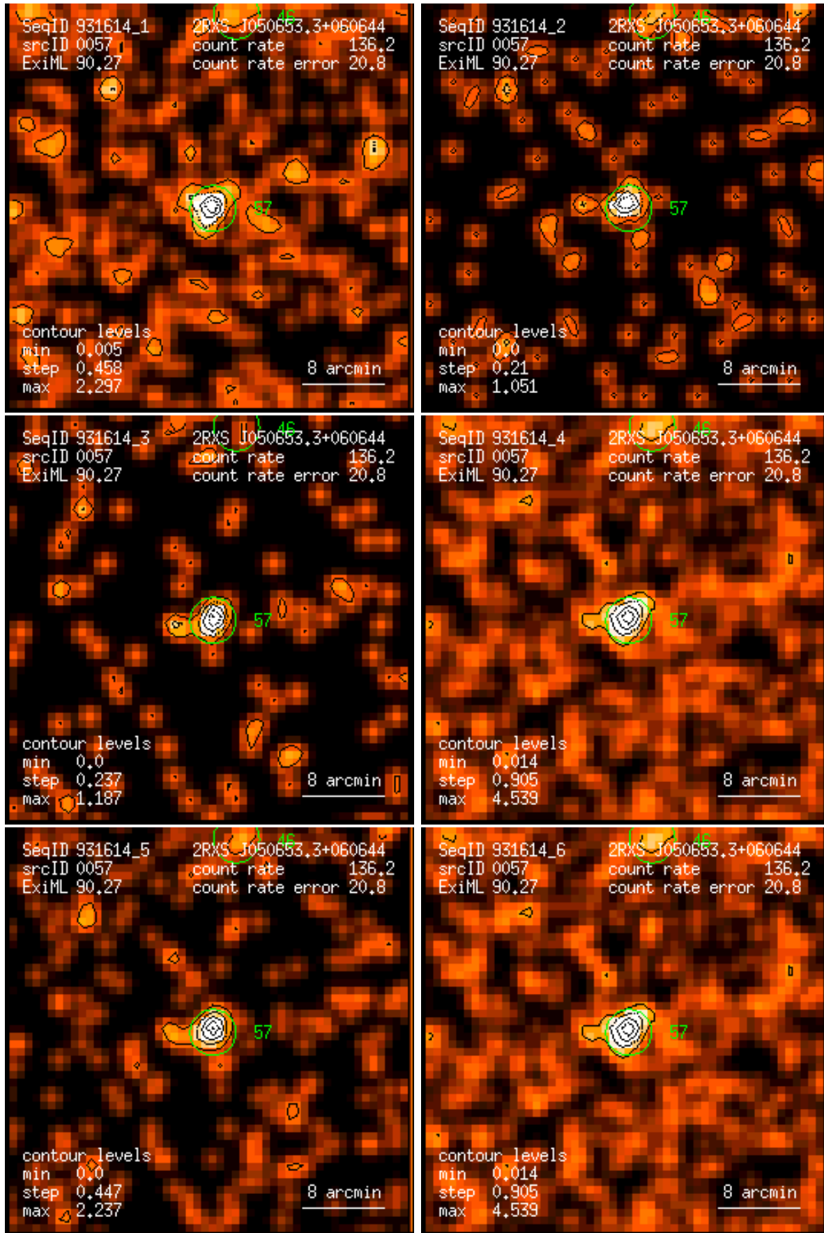
Figure 57: RASS 931614: detection 0057: band rate images, Gaussian filter: (1) PSPC channels 11 – 41, (2) 52 – 90, (3) 91 – 201, (4) 11 – 235, (5) 52 – 201, (6) 11 – 201. Broad band rates in counts/ks. Band rate contour levels in counts/ks/arcmin 2 .
