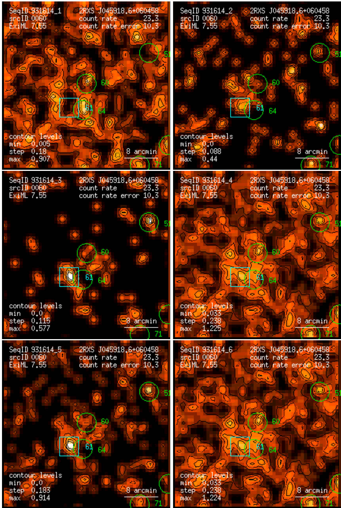
Figure 60: RASS 931614: detection 0060: band rate images, Gaussian filter: (1) PSPC channels 11 – 41, (2) 52 – 90, (3) 91 – 201, (4) 11 – 235, (5) 52 – 201, (6) 11 – 201. Broad band rates in counts/ks. Band rate contour levels in counts/ks/arcmin 2 .
