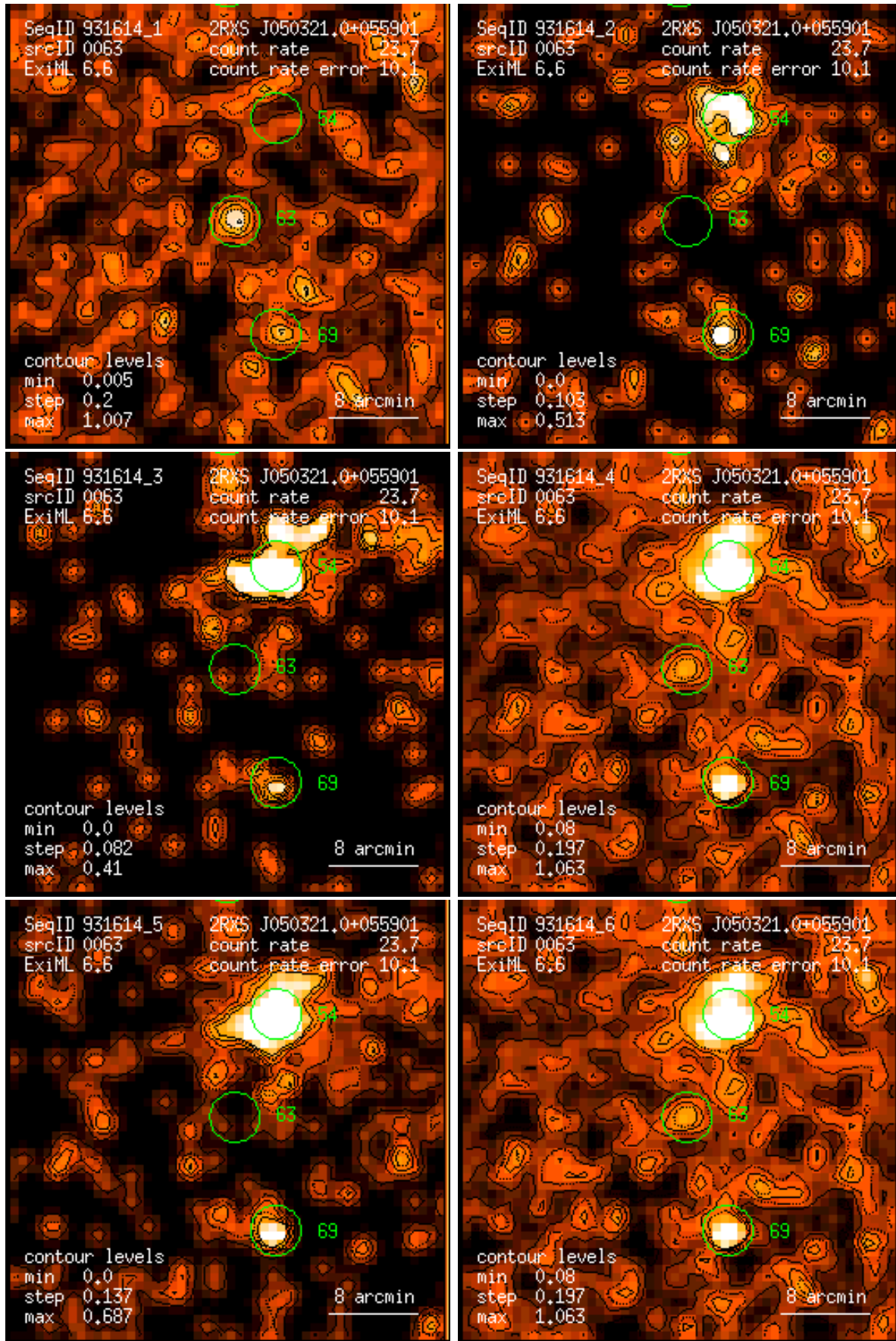
Figure 63: RASS 931614: detection 0063: band rate images, Gaussian filter: (1) PSPC channels 11 – 41, (2) 52 – 90, (3) 91 – 201, (4) 11 – 235, (5) 52 – 201, (6) 11 – 201. Broad band rates in counts/ks. Band rate contour levels in counts/ks/arcmin 2 .
