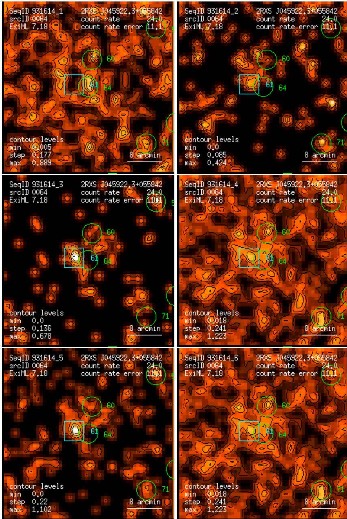
Figure 64: RASS 931614: detection 0064: band rate images, Gaussian filter: (1) PSPC channels 11 – 41, (2) 52 – 90, (3) 91 – 201, (4) 11 – 235, (5) 52 – 201, (6) 11 – 201. Broad band rates in counts/ks. Band rate contour levels in counts/ks/arcmin 2 .
