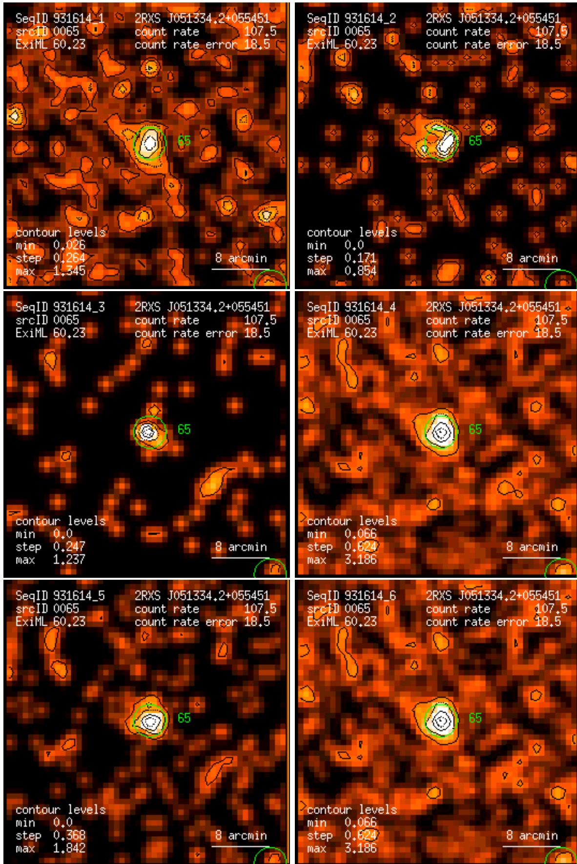
Figure 65: RASS 931614: detection 0065: band rate images, Gaussian filter: (1) PSPC channels 11 – 41, (2) 52 – 90, (3) 91 – 201, (4) 11 – 235, (5) 52 – 201, (6) 11 – 201. Broad band rates in counts/ks. Band rate contour levels in counts/ks/arcmin 2 .
