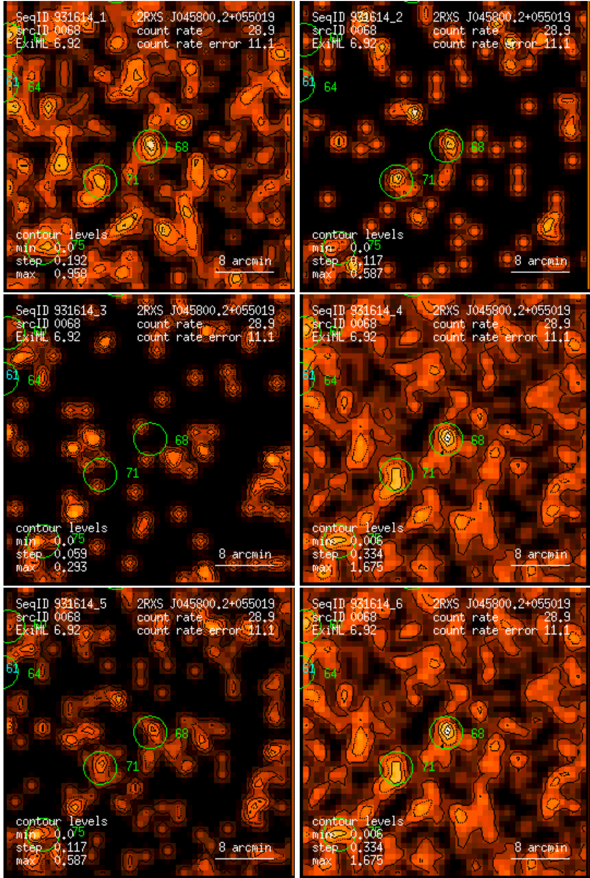
Figure 68: RASS 931614: detection 0068: band rate images, Gaussian filter: (1) PSPC channels 11 – 41, (2) 52 – 90, (3) 91 – 201, (4) 11 – 235, (5) 52 – 201, (6) 11 – 201. Broad band rates in counts/ks. Band rate contour levels in counts/ks/arcmin 2 .
