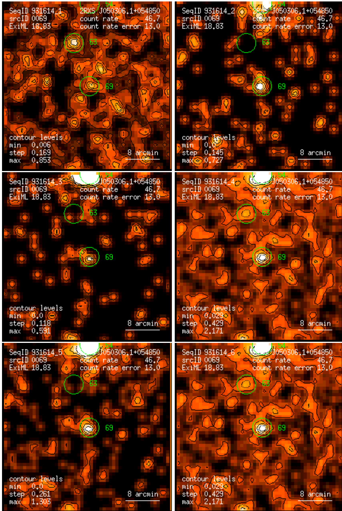
Figure 69: RASS 931614: detection 0069: band rate images, Gaussian filter: (1) PSPC channels 11 – 41, (2) 52 – 90, (3) 91 – 201, (4) 11 – 235, (5) 52 – 201, (6) 11 – 201. Broad band rates in counts/ks. Band rate contour levels in counts/ks/arcmin 2 .
