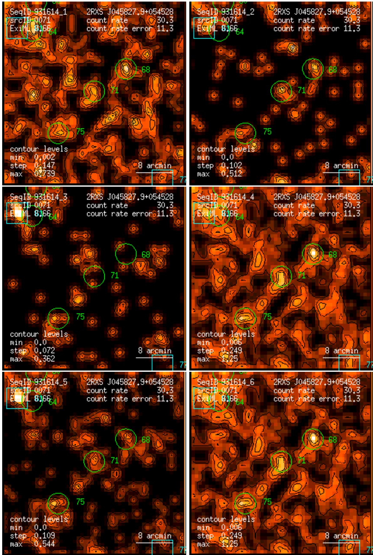
Figure 71: RASS 931614: detection 0071: band rate images, Gaussian filter: (1) PSPC channels 11 – 41, (2) 52 – 90, (3) 91 – 201, (4) 11 – 235, (5) 52 – 201, (6) 11 – 201. Broad band rates in counts/ks. Band rate contour levels in counts/ks/arcmin 2 .
