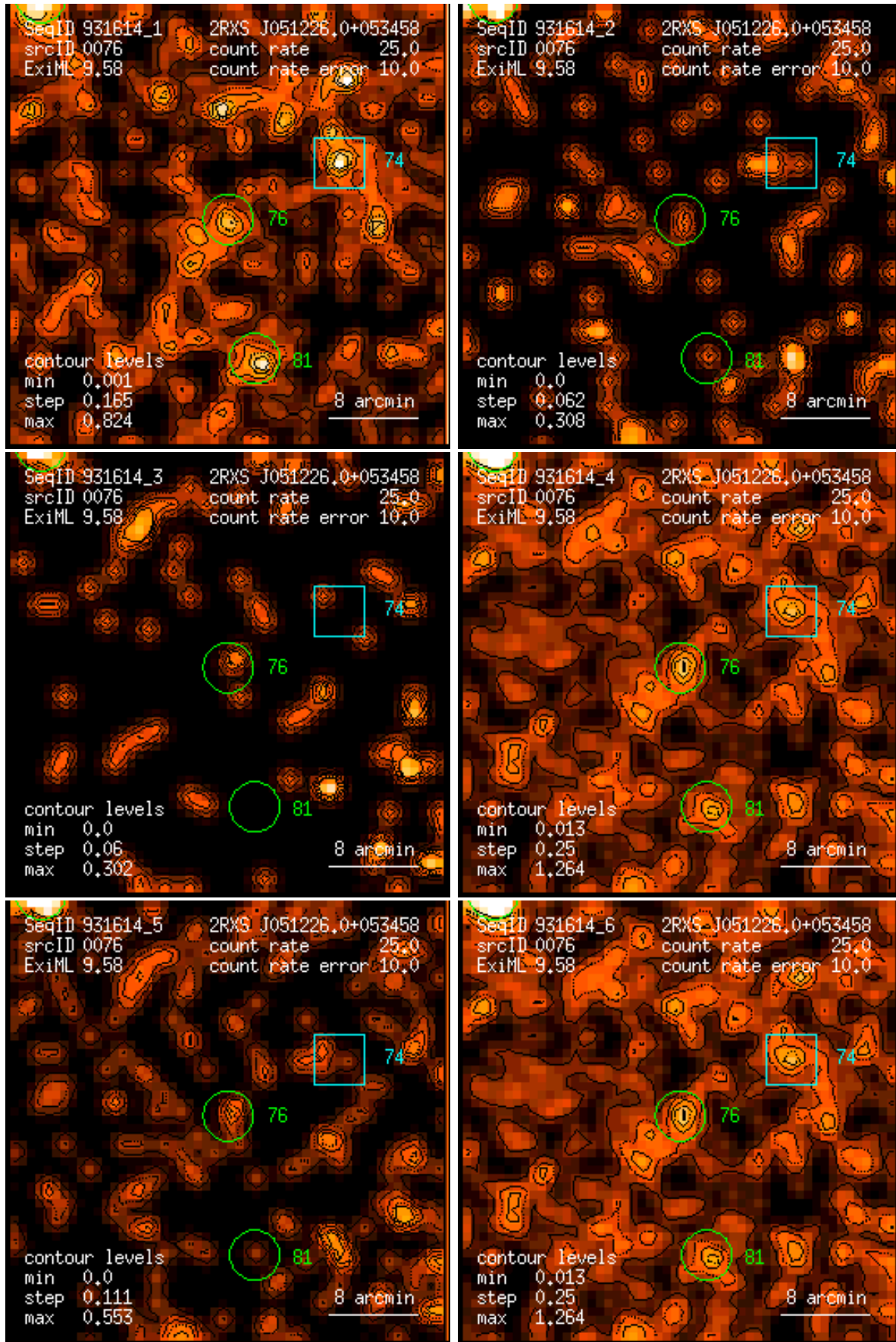
Figure 76: RASS 931614: detection 0076: band rate images, Gaussian filter: (1) PSPC channels 11 – 41, (2) 52 – 90, (3) 91 – 201, (4) 11 – 235, (5) 52 – 201, (6) 11 – 201. Broad band rates in counts/ks. Band rate contour levels in counts/ks/arcmin 2 .
