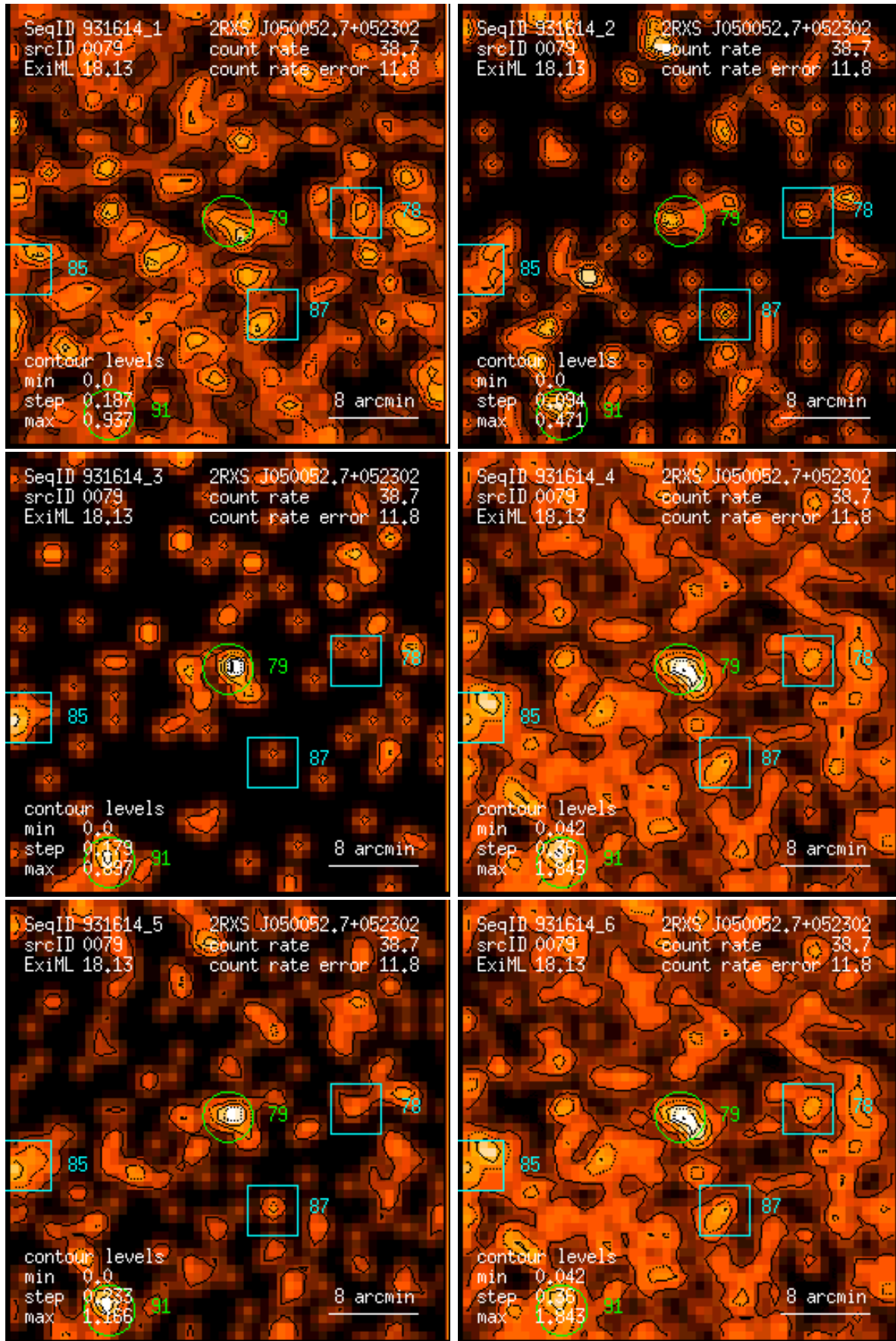
Figure 79: RASS 931614: detection 0079: band rate images, Gaussian filter: (1) PSPC channels 11 – 41, (2) 52 – 90, (3) 91 – 201, (4) 11 – 235, (5) 52 – 201, (6) 11 – 201. Broad band rates in counts/ks. Band rate contour levels in counts/ks/arcmin 2 .
