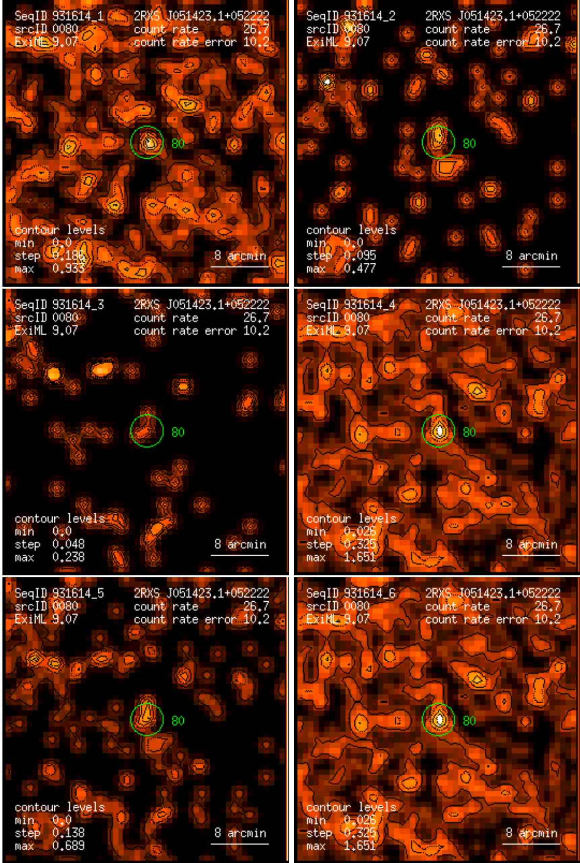
Figure 80: RASS 931614: detection 0080: band rate images, Gaussian filter: (1) PSPC channels 11 – 41, (2) 52 – 90, (3) 91 – 201, (4) 11 – 235, (5) 52 – 201, (6) 11 – 201. Broad band rates in counts/ks. Band rate contour levels in counts/ks/arcmin 2 .
