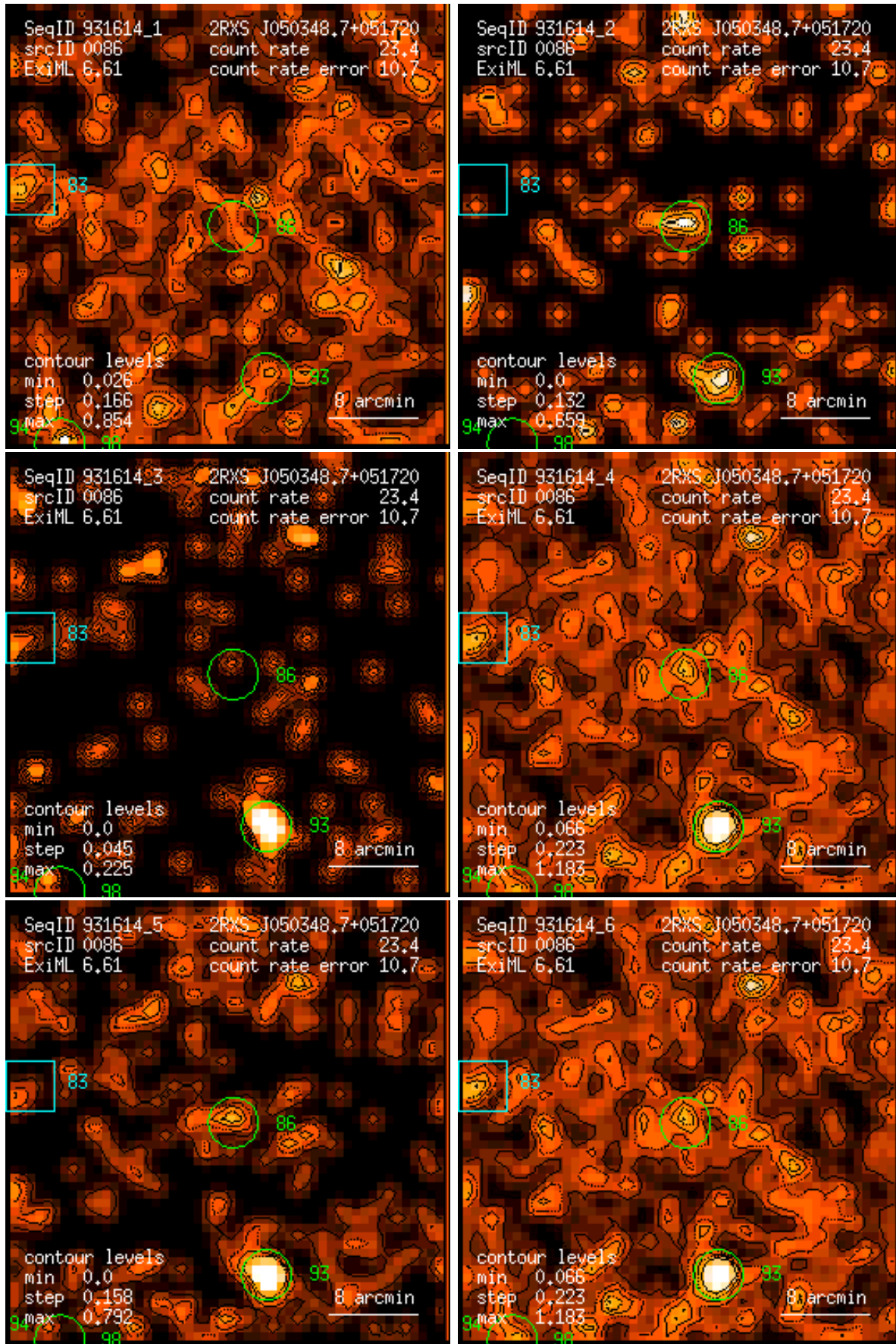
Figure 86: RASS 931614: detection 0086: band rate images, Gaussian filter: (1) PSPC channels 11 – 41, (2) 52 – 90, (3) 91 – 201, (4) 11 – 235, (5) 52 – 201, (6) 11 – 201. Broad band rates in counts/ks. Band rate contour levels in counts/ks/arcmin 2 .
