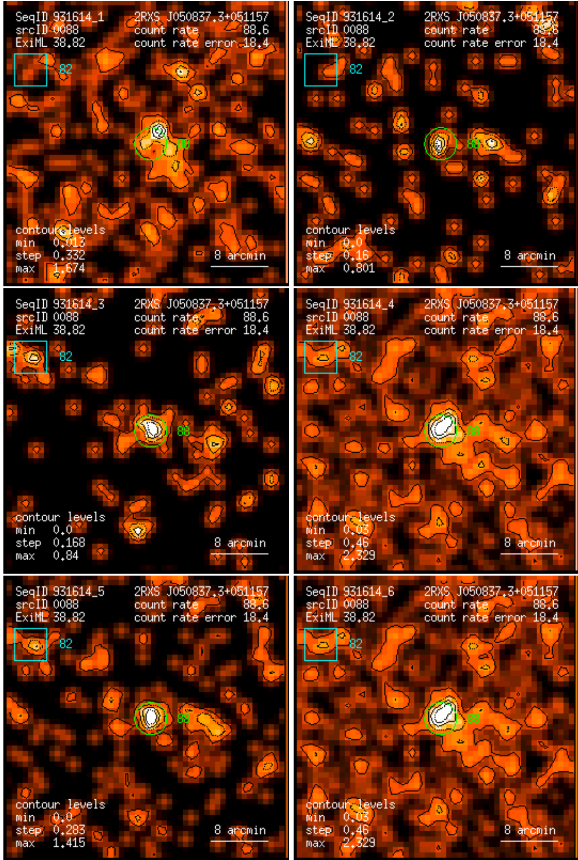
Figure 88: RASS 931614: detection 0088: band rate images, Gaussian filter: (1) PSPC channels 11 – 41, (2) 52 – 90, (3) 91 – 201, (4) 11 – 235, (5) 52 – 201, (6) 11 – 201. Broad band rates in counts/ks. Band rate contour levels in counts/ks/arcmin 2 .
