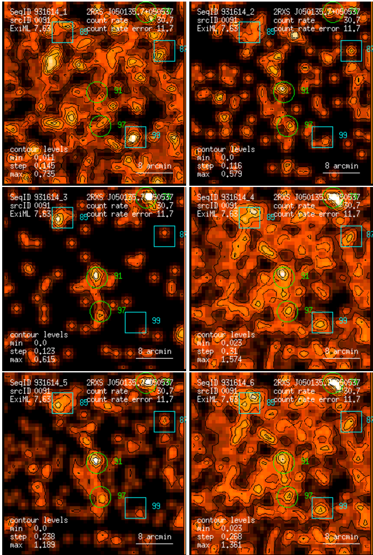
Figure 91: RASS 931614: detection 0091: band rate images, Gaussian filter: (1) PSPC channels 11 – 41, (2) 52 – 90, (3) 91 – 201, (4) 11 – 235, (5) 52 – 201, (6) 11 – 201. Broad band rates in counts/ks. Band rate contour levels in counts/ks/arcmin 2 .
