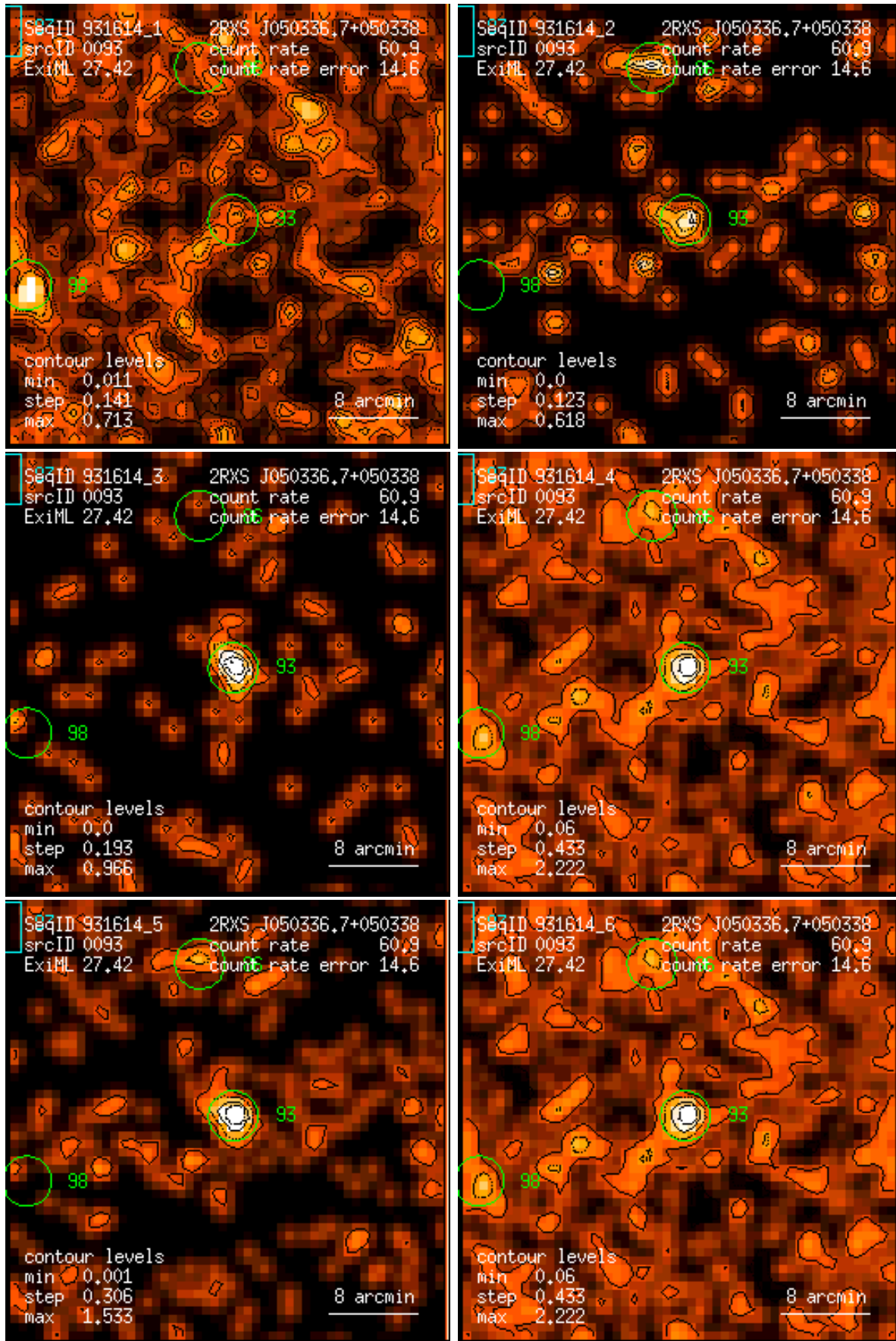
Figure 93: RASS 931614: detection 0093: band rate images, Gaussian filter: (1) PSPC channels 11 – 41, (2) 52 – 90, (3) 91 – 201, (4) 11 – 235, (5) 52 – 201, (6) 11 – 201. Broad band rates in counts/ks. Band rate contour levels in counts/ks/arcmin 2 .
