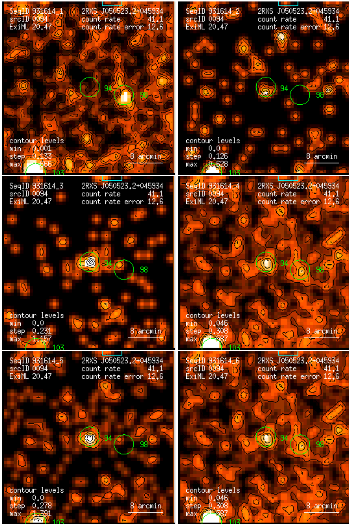
Figure 94: RASS 931614: detection 0094: band rate images, Gaussian filter: (1) PSPC channels 11 – 41, (2) 52 – 90, (3) 91 – 201, (4) 11 – 235, (5) 52 – 201, (6) 11 – 201. Broad band rates in counts/ks. Band rate contour levels in counts/ks/arcmin 2 .
