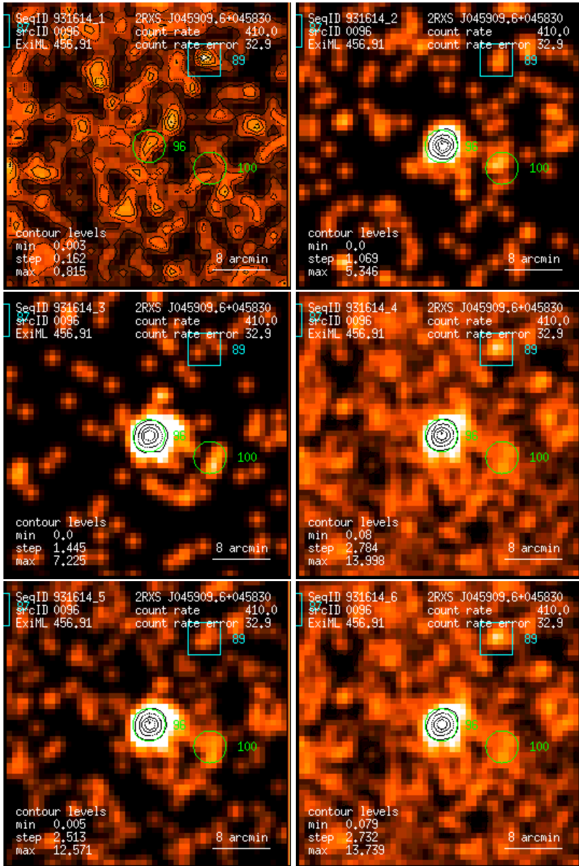
Figure 96: RASS 931614: detection 0096: band rate images, Gaussian filter: (1) PSPC channels 11 – 41, (2) 52 – 90, (3) 91 – 201, (4) 11 – 235, (5) 52 – 201, (6) 11 – 201. Broad band rates in counts/ks. Band rate contour levels in counts/ks/arcmin 2 .
