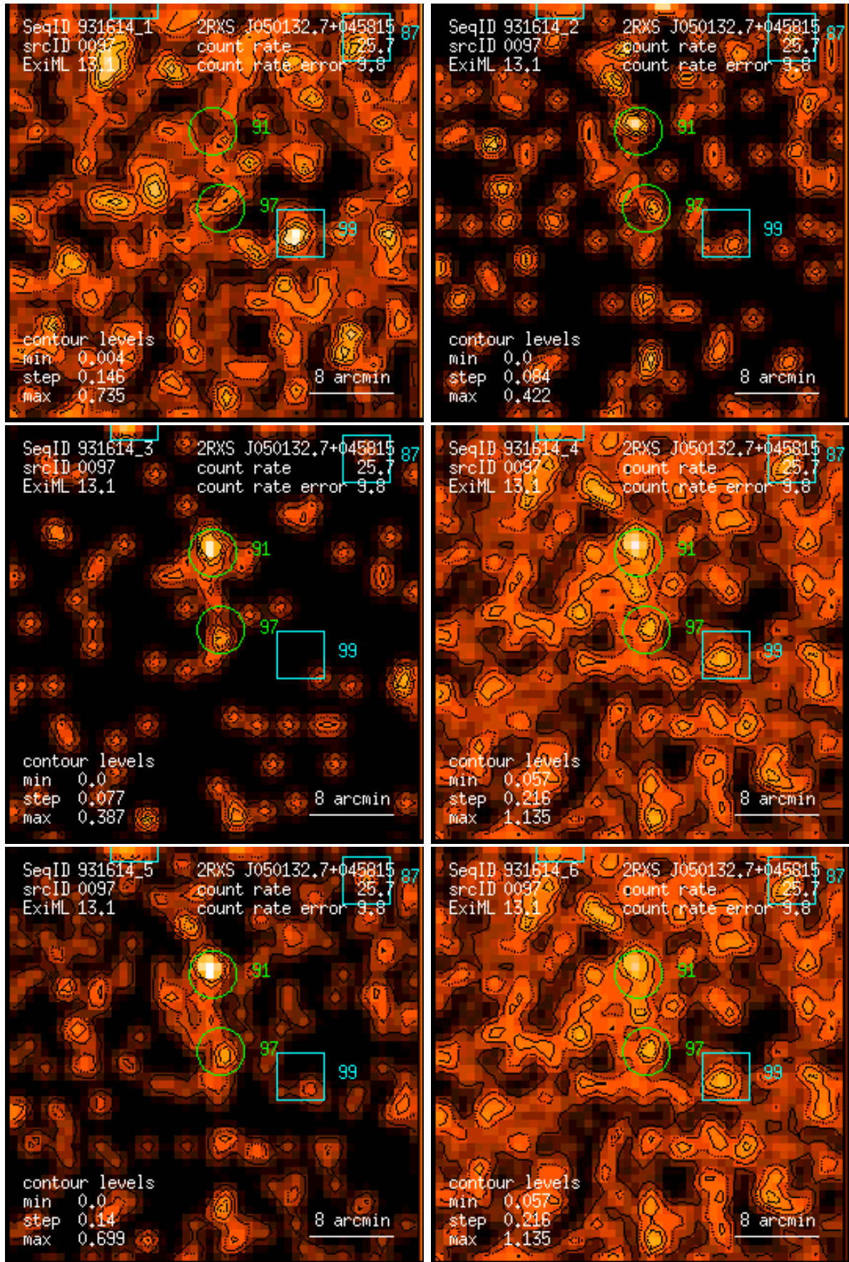
Figure 97: RASS 931614: detection 0097: band rate images, Gaussian filter: (1) PSPC channels 11 – 41, (2) 52 – 90, (3) 91 – 201, (4) 11 – 235, (5) 52 – 201, (6) 11 – 201. Broad band rates in counts/ks. Band rate contour levels in counts/ks/arcmin 2 .
