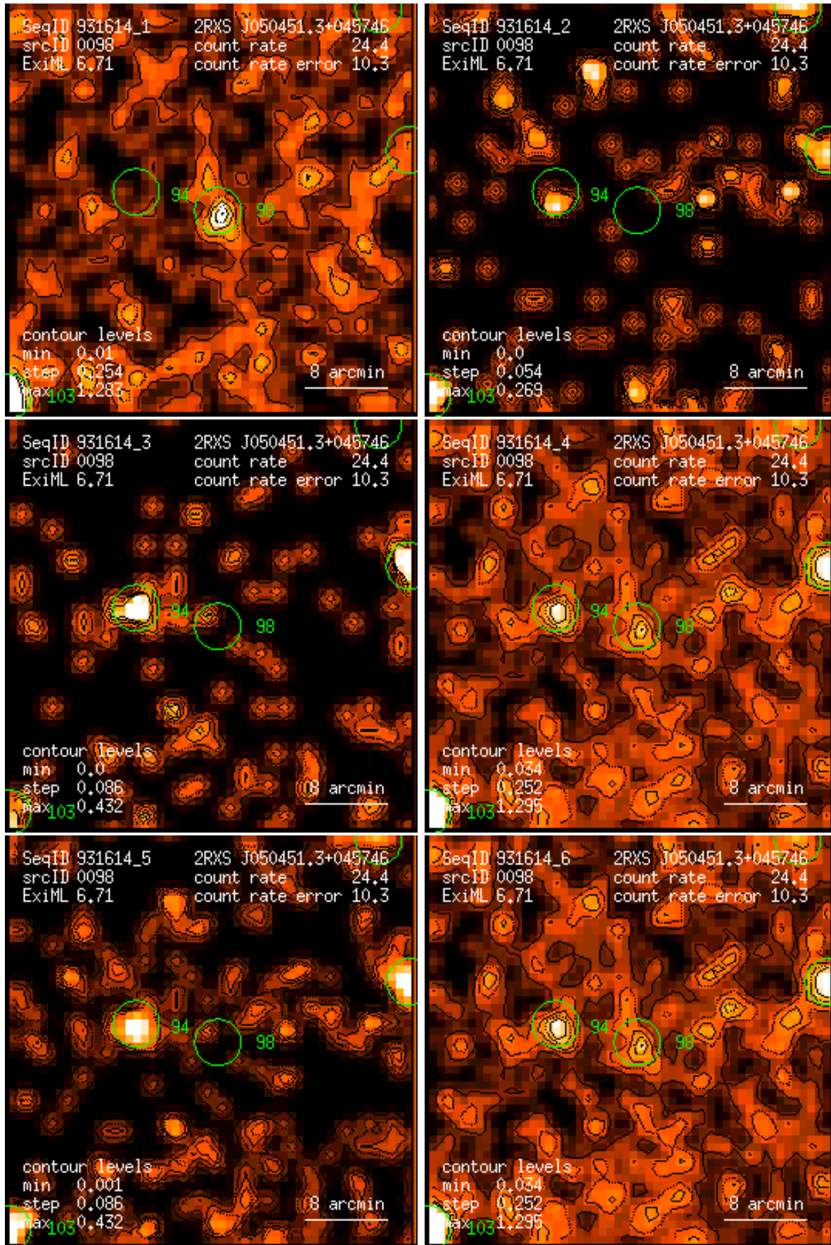
Figure 98: RASS 931614: detection 0098: band rate images, Gaussian filter: (1) PSPC channels 11 – 41, (2) 52 – 90, (3) 91 – 201, (4) 11 – 235, (5) 52 – 201, (6) 11 – 201. Broad band rates in counts/ks. Band rate contour levels in counts/ks/arcmin 2 .
