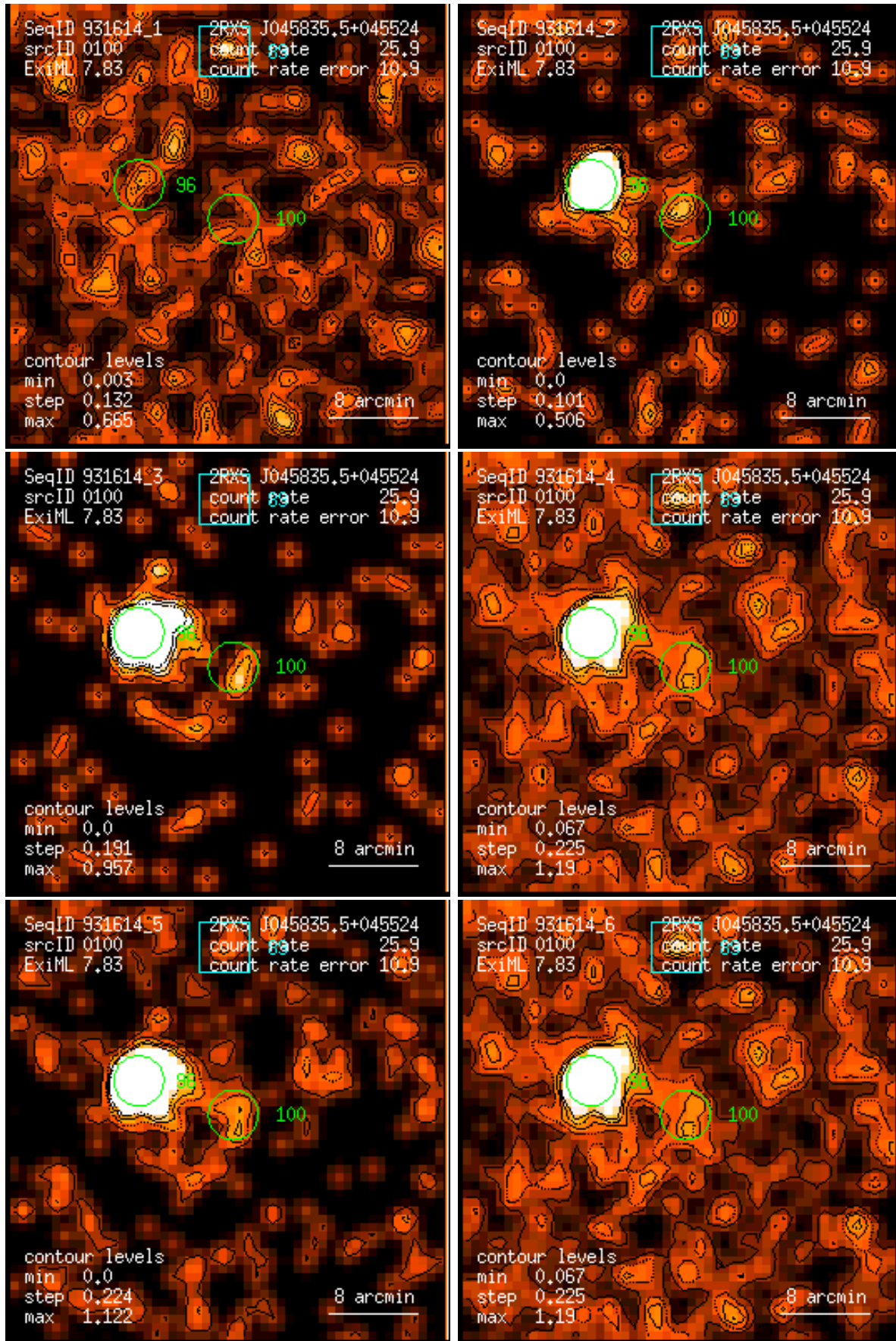
Figure 100: RASS 931614: detection 0100: band rate images, Gaussian filter: (1) PSPC channels 11 – 41, (2) 52 – 90, (3) 91 – 201, (4) 11 – 235, (5) 52 – 201, (6) 11 – 201. Broad band rates in counts/ks. Band rate contour levels in counts/ks/arcmin 2 .
