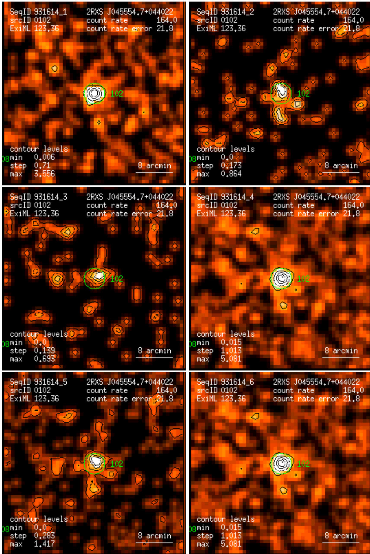
Figure 102: RASS 931614: detection 0102: band rate images, Gaussian filter: (1) PSPC channels 11 – 41, (2) 52 – 90, (3) 91 – 201, (4) 11 – 235, (5) 52 – 201, (6) 11 – 201. Broad band rates in counts/ks. Band rate contour levels in counts/ks/arcmin 2 .
