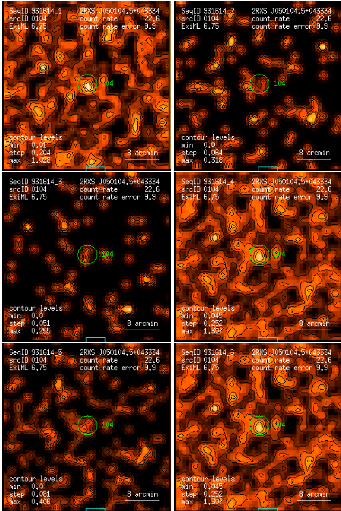
Figure 104: RASS 931614: detection 0104: band rate images, Gaussian filter: (1) PSPC channels 11 – 41, (2) 52 – 90, (3) 91 – 201, (4) 11 – 235, (5) 52 – 201, (6) 11 – 201. Broad band rates in counts/ks. Band rate contour levels in counts/ks/arcmin 2 .
