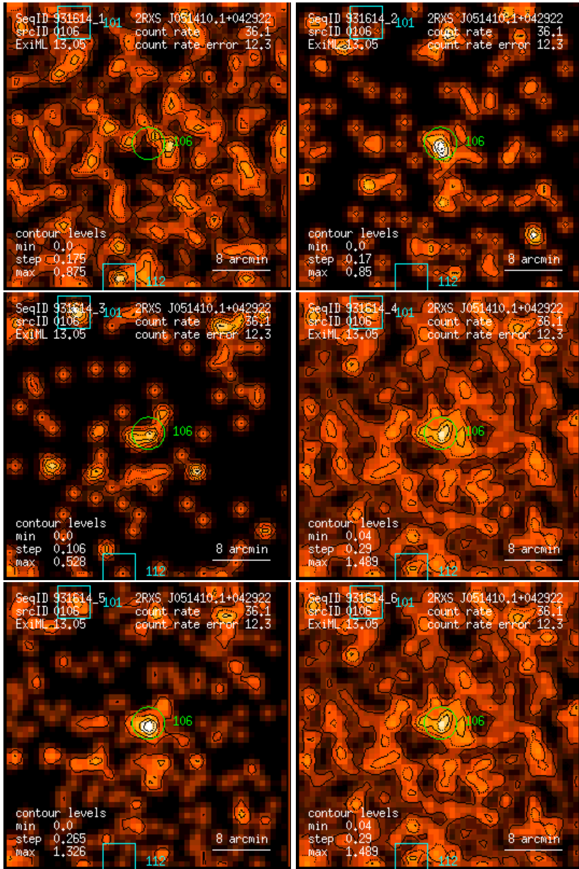
Figure 106: RASS 931614: detection 0106: band rate images, Gaussian filter: (1) PSPC channels 11 – 41, (2) 52 – 90, (3) 91 – 201, (4) 11 – 235, (5) 52 – 201, (6) 11 – 201. Broad band rates in counts/ks. Band rate contour levels in counts/ks/arcmin 2 .
