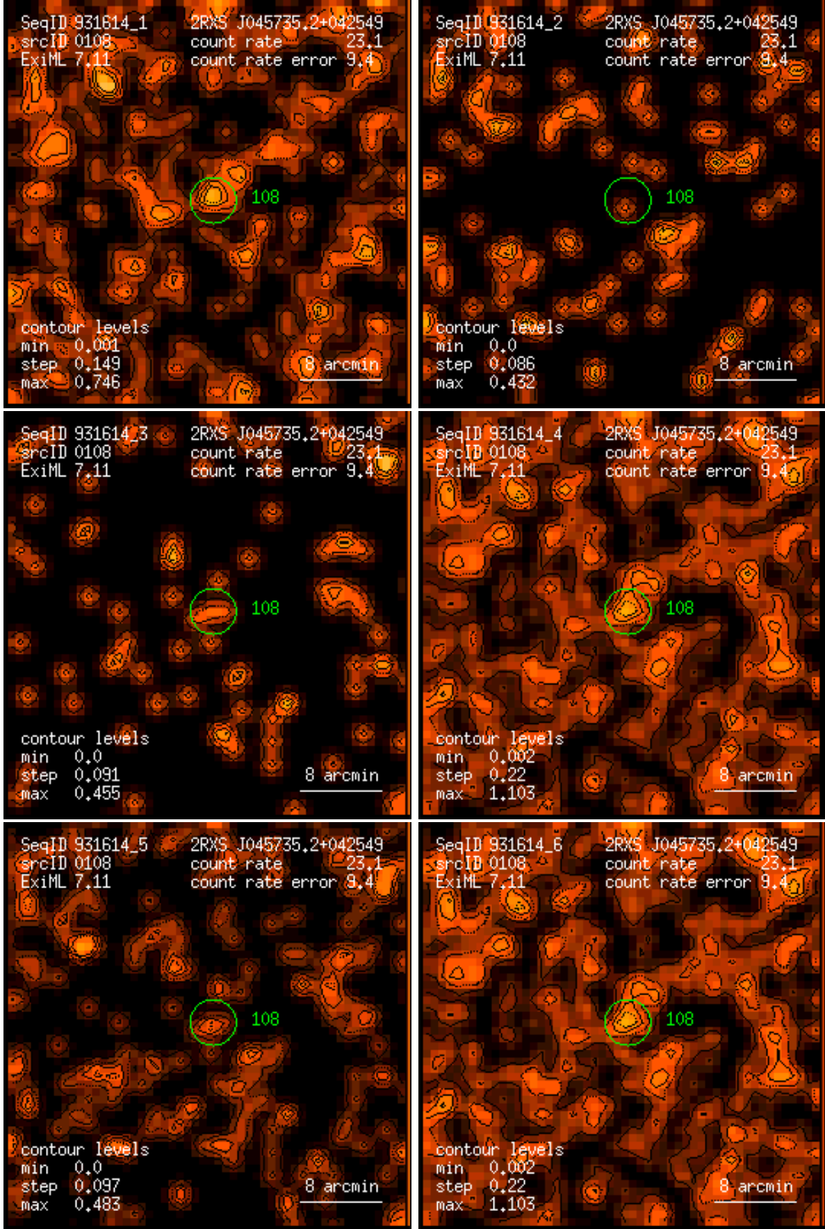
Figure 108: RASS 931614: detection 0108: band rate images, Gaussian filter: (1) PSPC channels 11 – 41, (2) 52 – 90, (3) 91 – 201, (4) 11 – 235, (5) 52 – 201, (6) 11 – 201. Broad band rates in counts/ks. Band rate contour levels in counts/ks/arcmin 2 .
