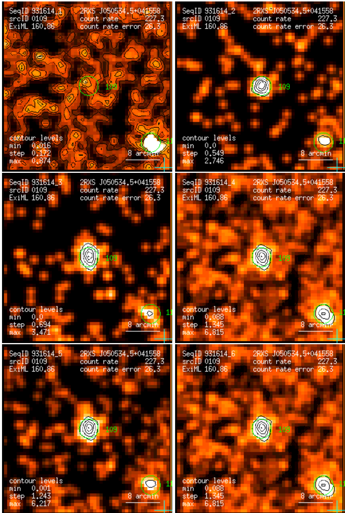
Figure 109: RASS 931614: detection 0109: band rate images, Gaussian filter: (1) PSPC channels 11 – 41, (2) 52 – 90, (3) 91 – 201, (4) 11 – 235, (5) 52 – 201, (6) 11 – 201. Broad band rates in counts/ks. Band rate contour levels in counts/ks/arcmin 2 .
