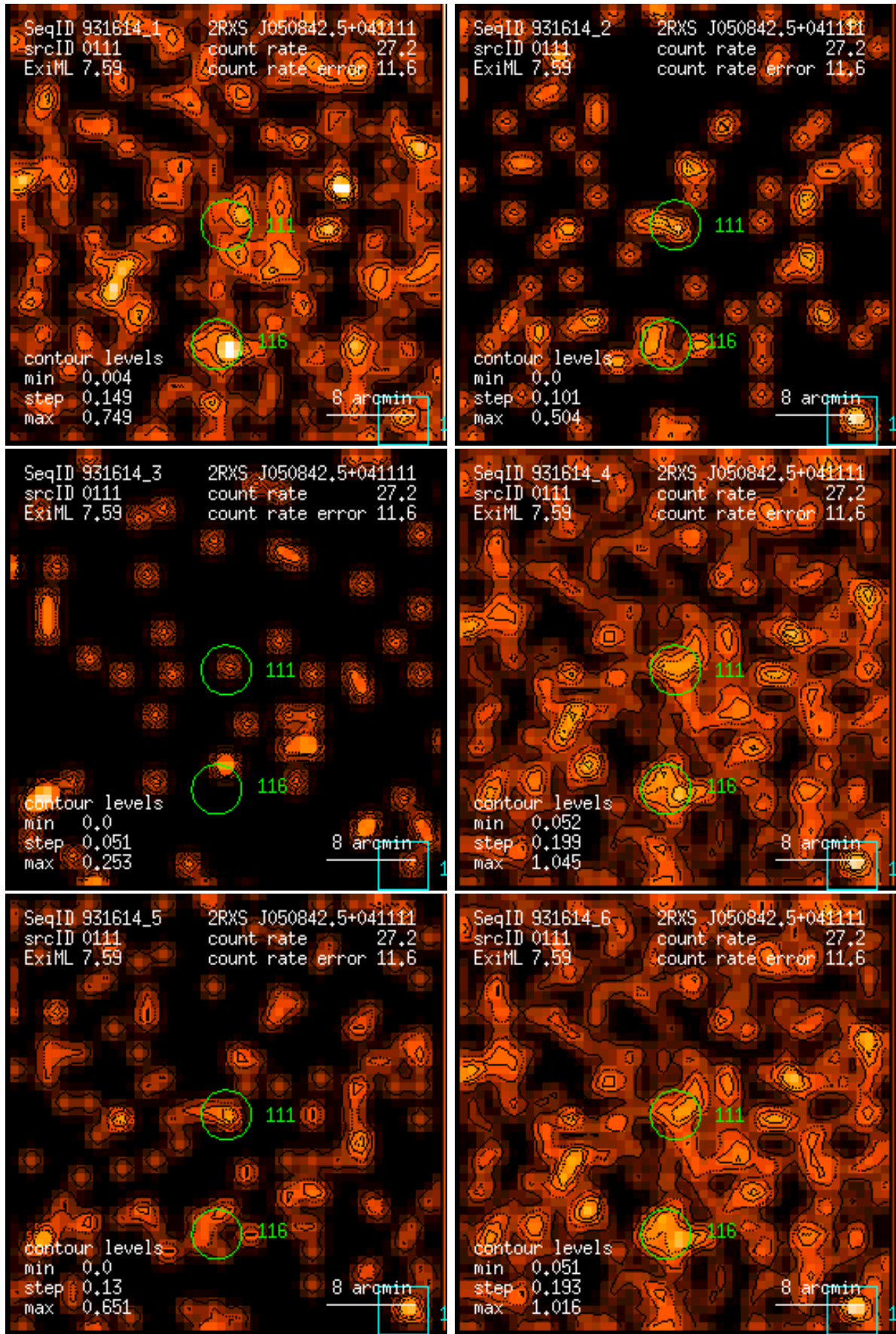
Figure 111: RASS 931614: detection 0111: band rate images, Gaussian filter: (1) PSPC channels 11 – 41, (2) 52 – 90, (3) 91 – 201, (4) 11 – 235, (5) 52 – 201, (6) 11 – 201. Broad band rates in counts/ks. Band rate contour levels in counts/ks/arcmin 2 .
