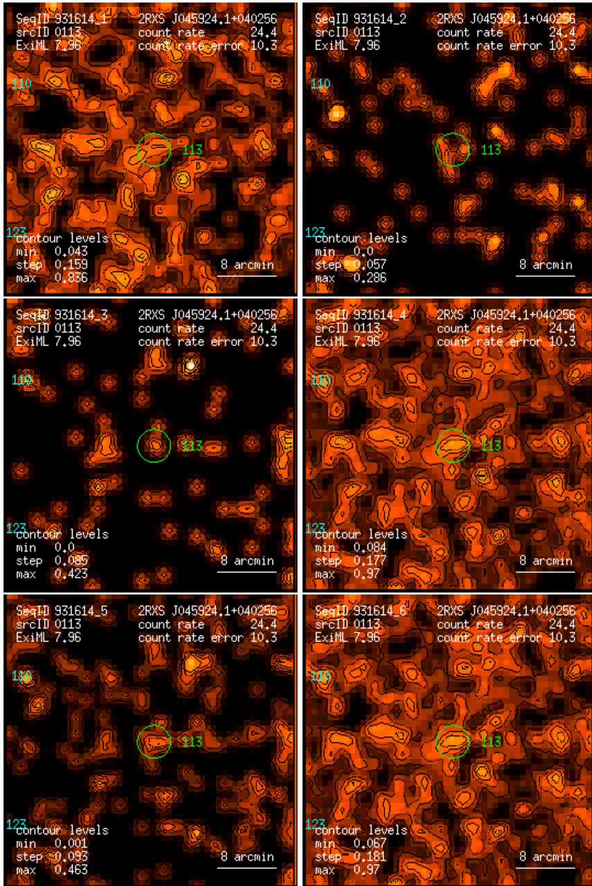
Figure 113: RASS 931614: detection 0113: band rate images, Gaussian filter: (1) PSPC channels 11 – 41, (2) 52 – 90, (3) 91 – 201, (4) 11 – 235, (5) 52 – 201, (6) 11 – 201. Broad band rates in counts/ks. Band rate contour levels in counts/ks/arcmin 2 .
