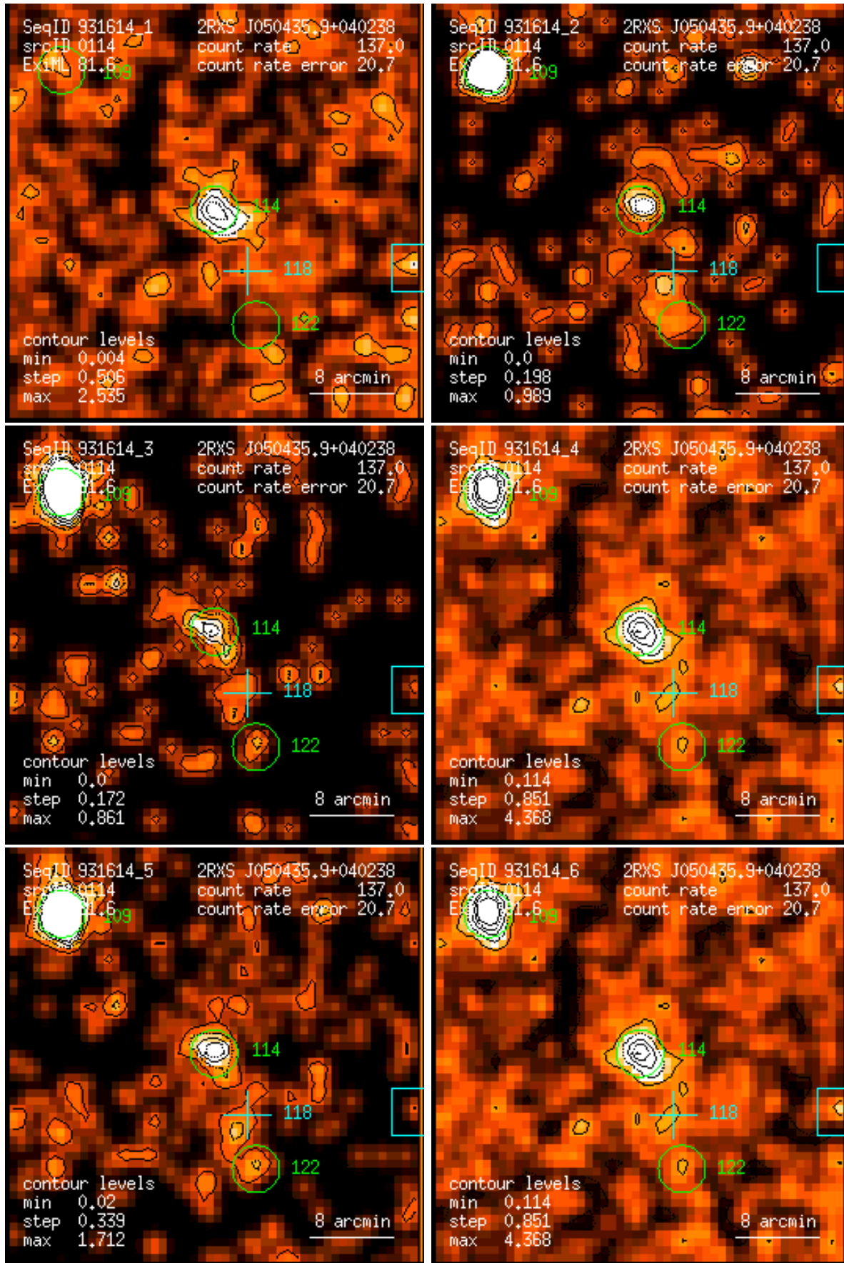
Figure 114: RASS 931614: detection 0114: band rate images, Gaussian filter: (1) PSPC channels 11 – 41, (2) 52 – 90, (3) 91 – 201, (4) 11 – 235, (5) 52 – 201, (6) 11 – 201. Broad band rates in counts/ks. Band rate contour levels in counts/ks/arcmin 2 .
