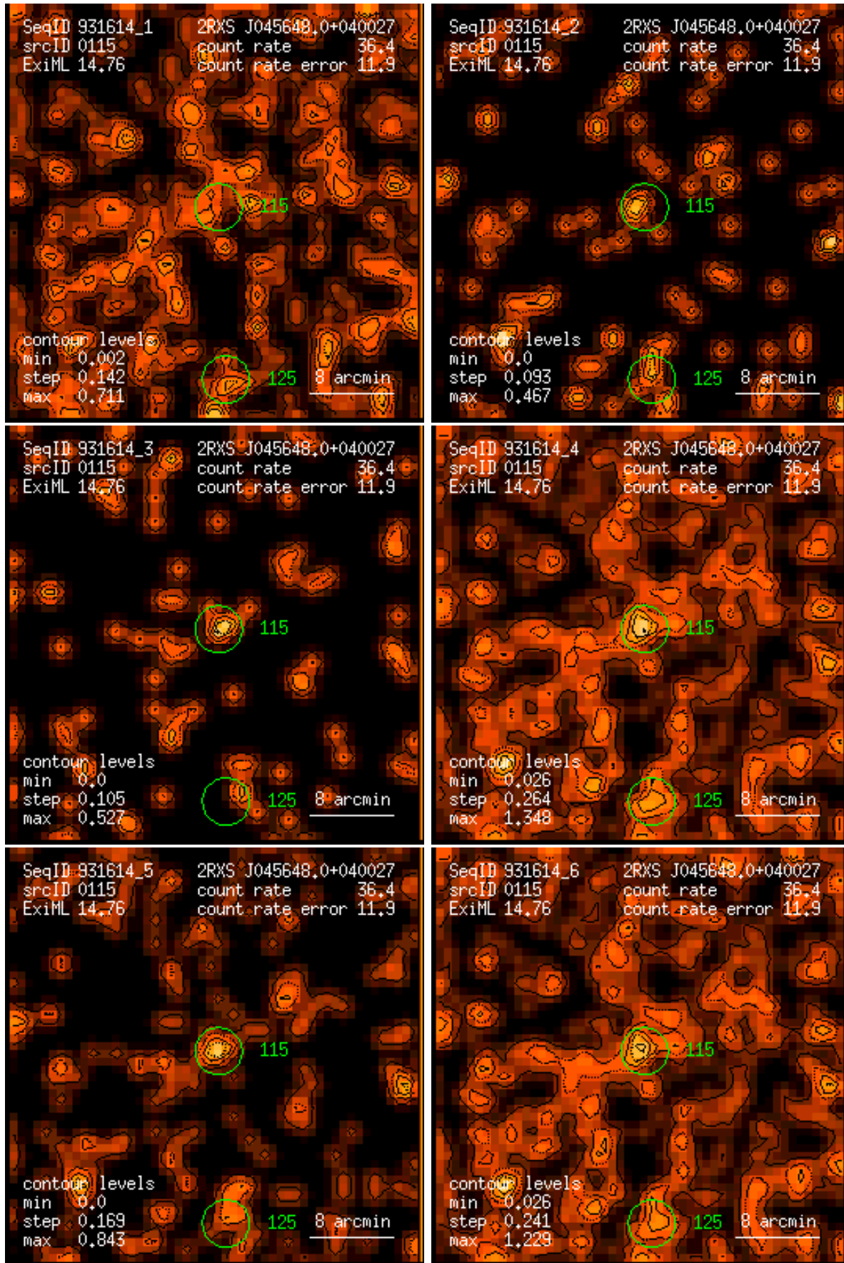
Figure 115: RASS 931614: detection 0115: band rate images, Gaussian filter: (1) PSPC channels 11 – 41, (2) 52 – 90, (3) 91 – 201, (4) 11 – 235, (5) 52 – 201, (6) 11 – 201. Broad band rates in counts/ks. Band rate contour levels in counts/ks/arcmin 2 .
