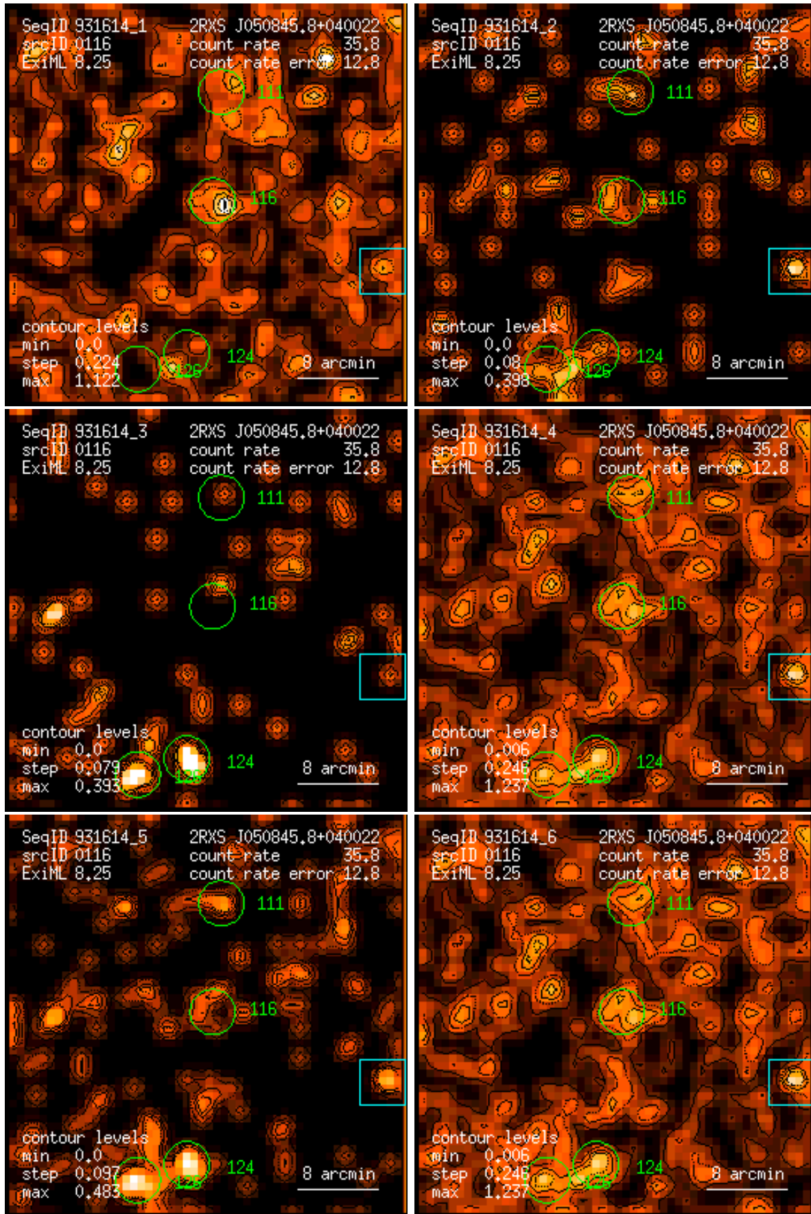
Figure 116: RASS 931614: detection 0116: band rate images, Gaussian filter: (1) PSPC channels 11 – 41, (2) 52 – 90, (3) 91 – 201, (4) 11 – 235, (5) 52 – 201, (6) 11 – 201. Broad band rates in counts/ks. Band rate contour levels in counts/ks/arcmin 2 .
