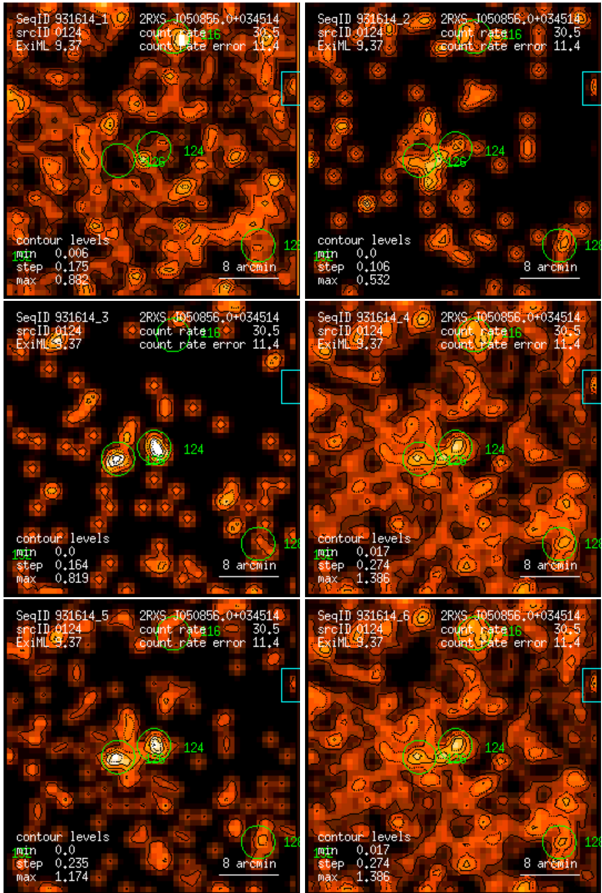
Figure 124: RASS 931614: detection 0124: band rate images, Gaussian filter: (1) PSPC channels 11 – 41, (2) 52 – 90, (3) 91 – 201, (4) 11 – 235, (5) 52 – 201, (6) 11 – 201. Broad band rates in counts/ks. Band rate contour levels in counts/ks/arcmin 2 .
