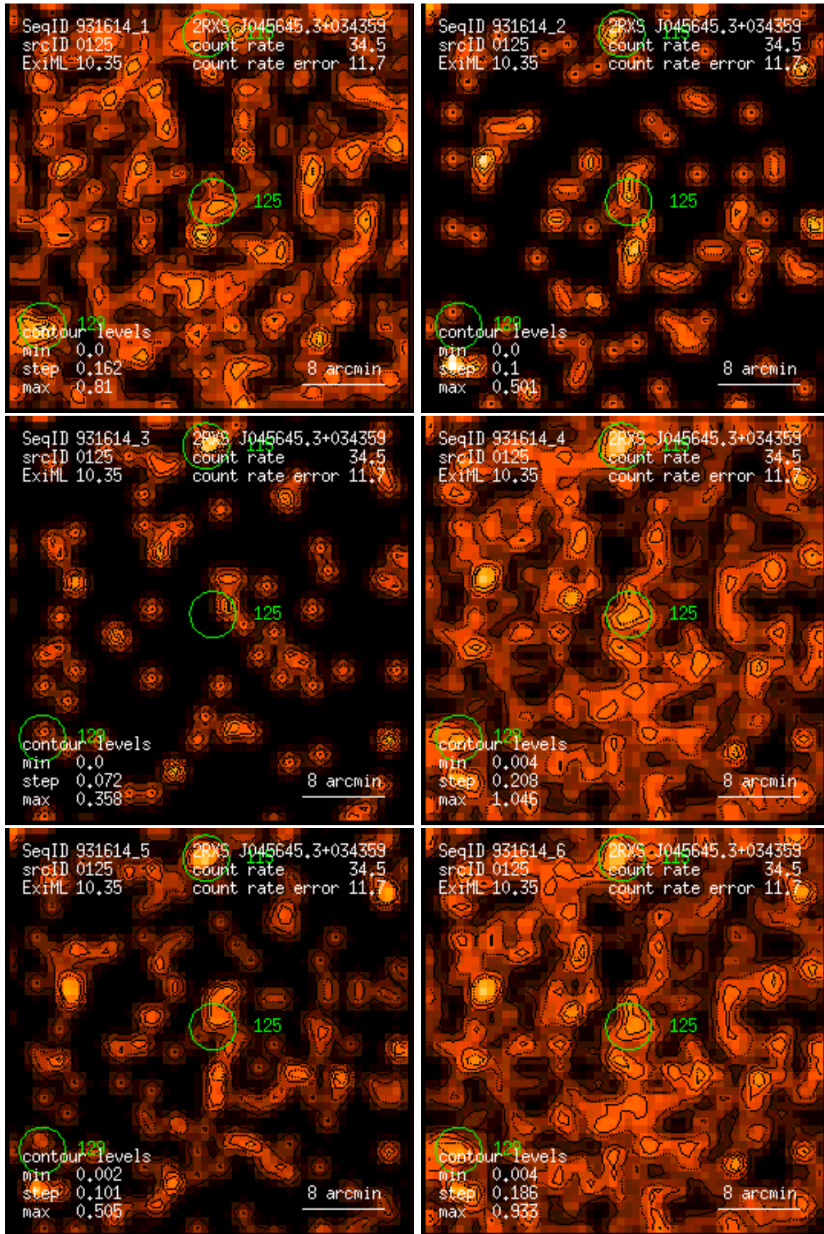
Figure 125: RASS 931614: detection 0125: band rate images, Gaussian filter: (1) PSPC channels 11 – 41, (2) 52 – 90, (3) 91 – 201, (4) 11 – 235, (5) 52 – 201, (6) 11 – 201. Broad band rates in counts/ks. Band rate contour levels in counts/ks/arcmin 2 .
