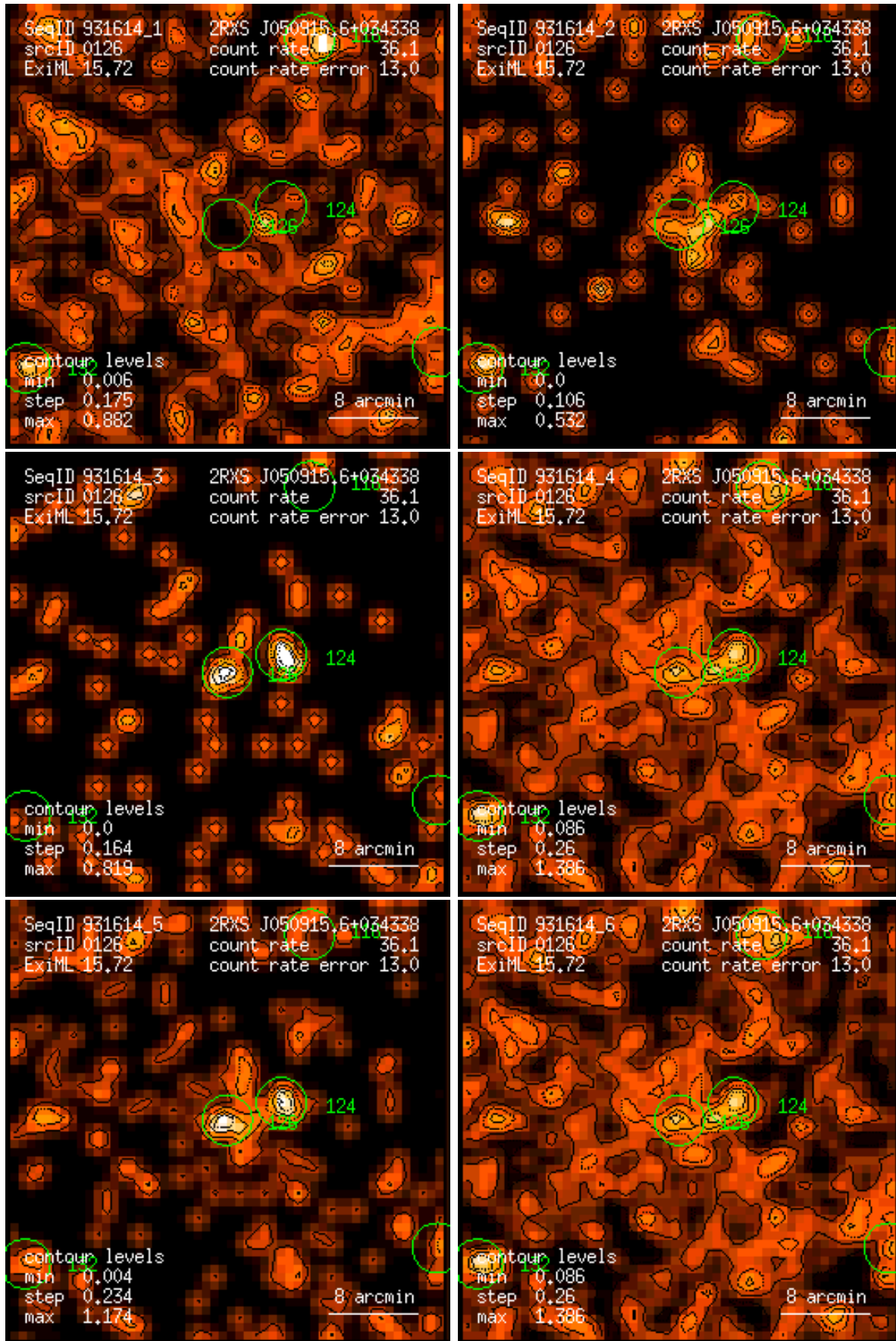
Figure 126: RASS 931614: detection 0126: band rate images, Gaussian filter: (1) PSPC channels 11 – 41, (2) 52 – 90, (3) 91 – 201, (4) 11 – 235, (5) 52 – 201, (6) 11 – 201. Broad band rates in counts/ks. Band rate contour levels in counts/ks/arcmin 2 .
