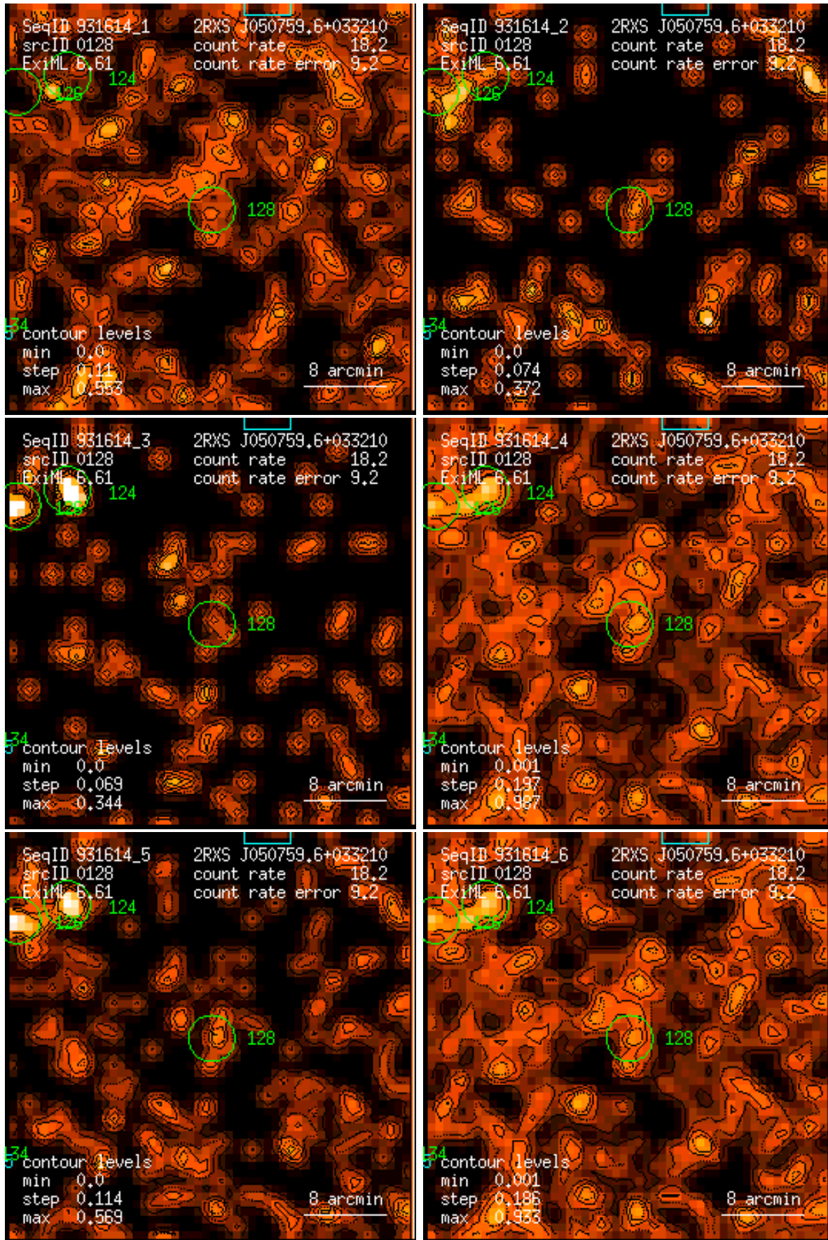
Figure 128: RASS 931614: detection 0128: band rate images, Gaussian filter: (1) PSPC channels 11 – 41, (2) 52 – 90, (3) 91 – 201, (4) 11 – 235, (5) 52 – 201, (6) 11 – 201. Broad band rates in counts/ks. Band rate contour levels in counts/ks/arcmin 2 .
