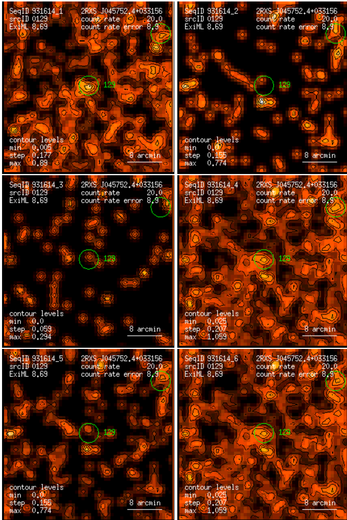
Figure 129: RASS 931614: detection 0129: band rate images, Gaussian filter: (1) PSPC channels 11 – 41, (2) 52 – 90, (3) 91 – 201, (4) 11 – 235, (5) 52 – 201, (6) 11 – 201. Broad band rates in counts/ks. Band rate contour levels in counts/ks/arcmin 2 .
