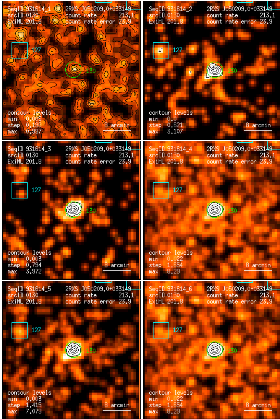
Figure 130: RASS 931614: detection 0130: band rate images, Gaussian filter: (1) PSPC channels 11 – 41, (2) 52 – 90, (3) 91 – 201, (4) 11 – 235, (5) 52 – 201, (6) 11 – 201. Broad band rates in counts/ks. Band rate contour levels in counts/ks/arcmin 2 .
