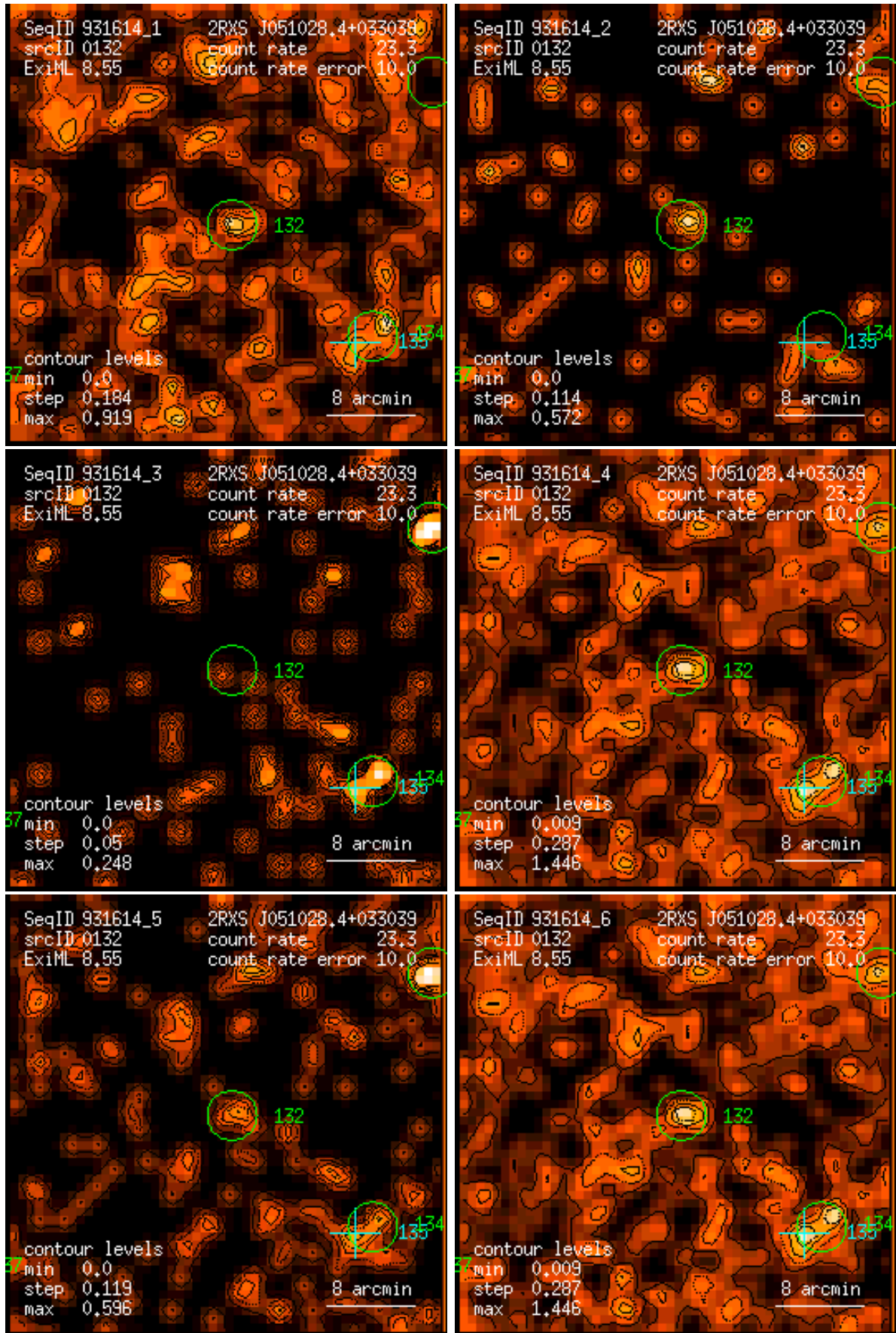
Figure 132: RASS 931614: detection 0132: band rate images, Gaussian filter: (1) PSPC channels 11 – 41, (2) 52 – 90, (3) 91 – 201, (4) 11 – 235, (5) 52 – 201, (6) 11 – 201. Broad band rates in counts/ks. Band rate contour levels in counts/ks/arcmin 2 .
