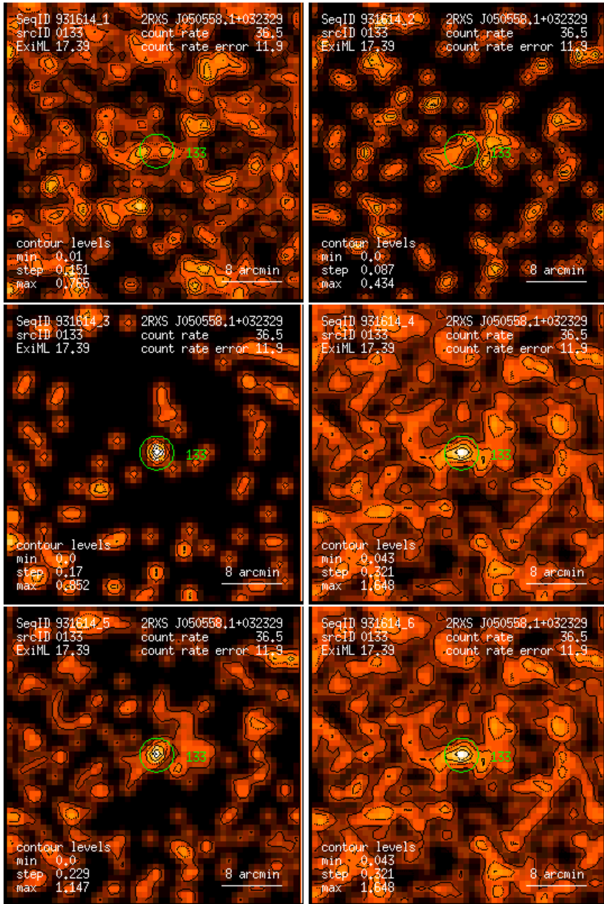
Figure 133: RASS 931614: detection 0133: band rate images, Gaussian filter: (1) PSPC channels 11 – 41, (2) 52 – 90, (3) 91 – 201, (4) 11 – 235, (5) 52 – 201, (6) 11 – 201. Broad band rates in counts/ks. Band rate contour levels in counts/ks/arcmin 2 .
