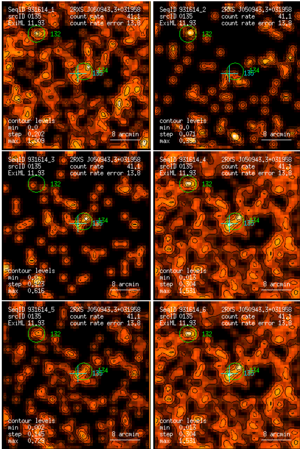
Figure 135: RASS 931614: detection 0135: band rate images, Gaussian filter: (1) PSPC channels 11 – 41, (2) 52 – 90, (3) 91 – 201, (4) 11 – 235, (5) 52 – 201, (6) 11 – 201. Broad band rates in counts/ks. Band rate contour levels in counts/ks/arcmin 2 .
