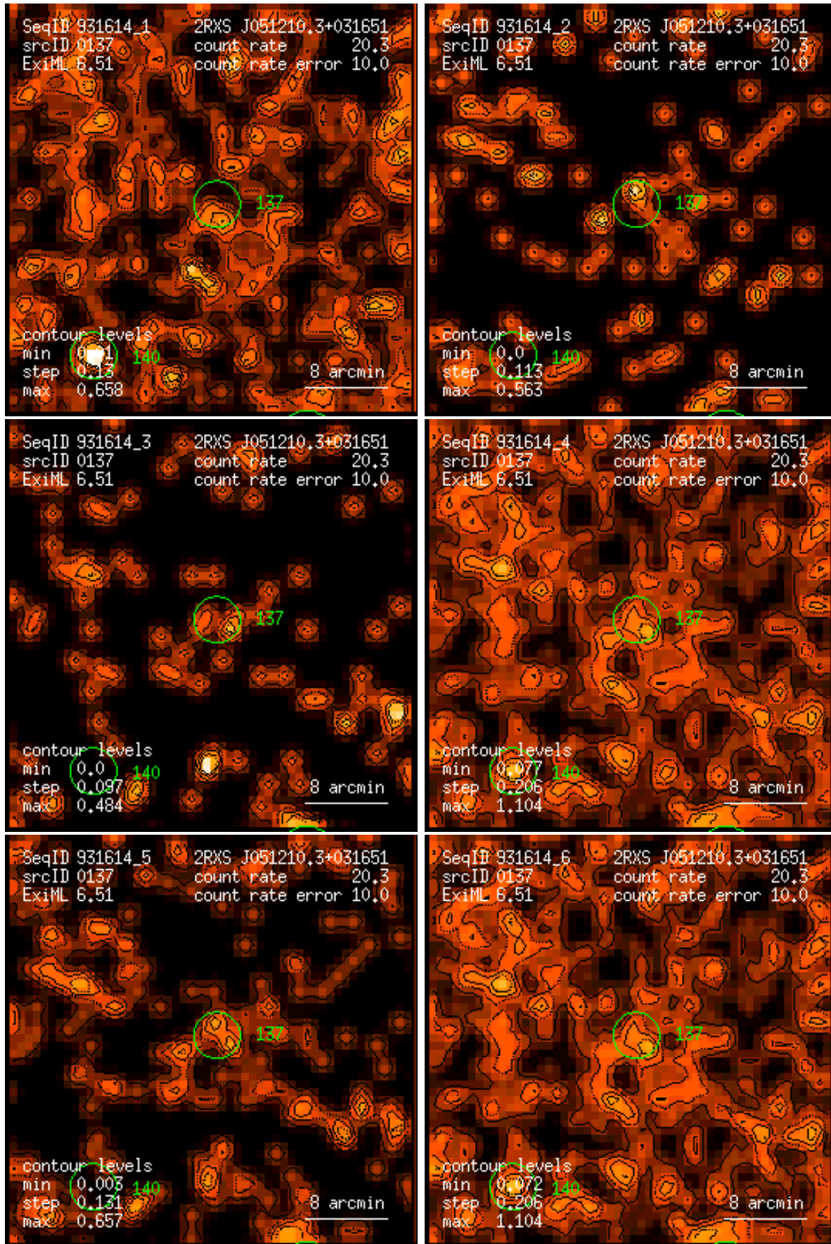
Figure 137: RASS 931614: detection 0137: band rate images, Gaussian filter: (1) PSPC channels 11 – 41, (2) 52 – 90, (3) 91 – 201, (4) 11 – 235, (5) 52 – 201, (6) 11 – 201. Broad band rates in counts/ks. Band rate contour levels in counts/ks/arcmin 2 .
