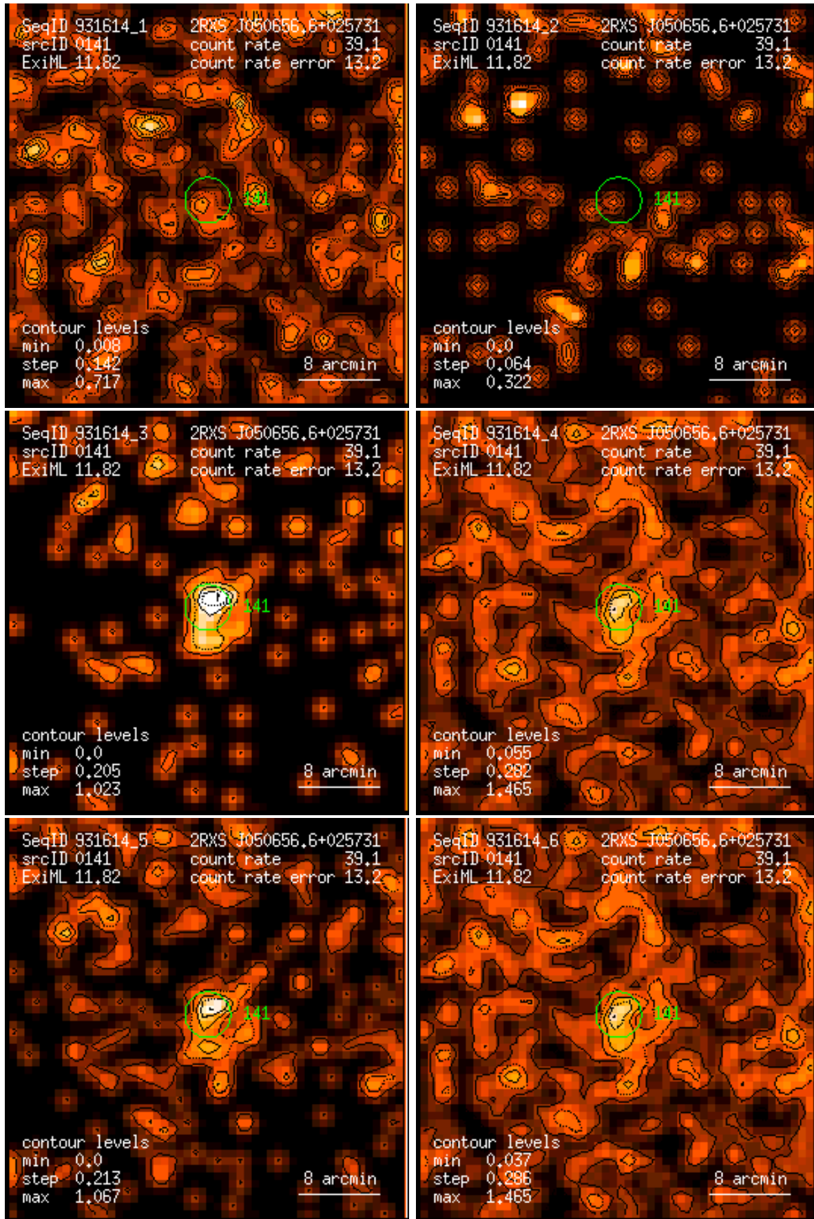
Figure 141: RASS 931614: detection 0141: band rate images, Gaussian filter: (1) PSPC channels 11 – 41, (2) 52 – 90, (3) 91 – 201, (4) 11 – 235, (5) 52 – 201, (6) 11 – 201. Broad band rates in counts/ks. Band rate contour levels in counts/ks/arcmin 2 .
