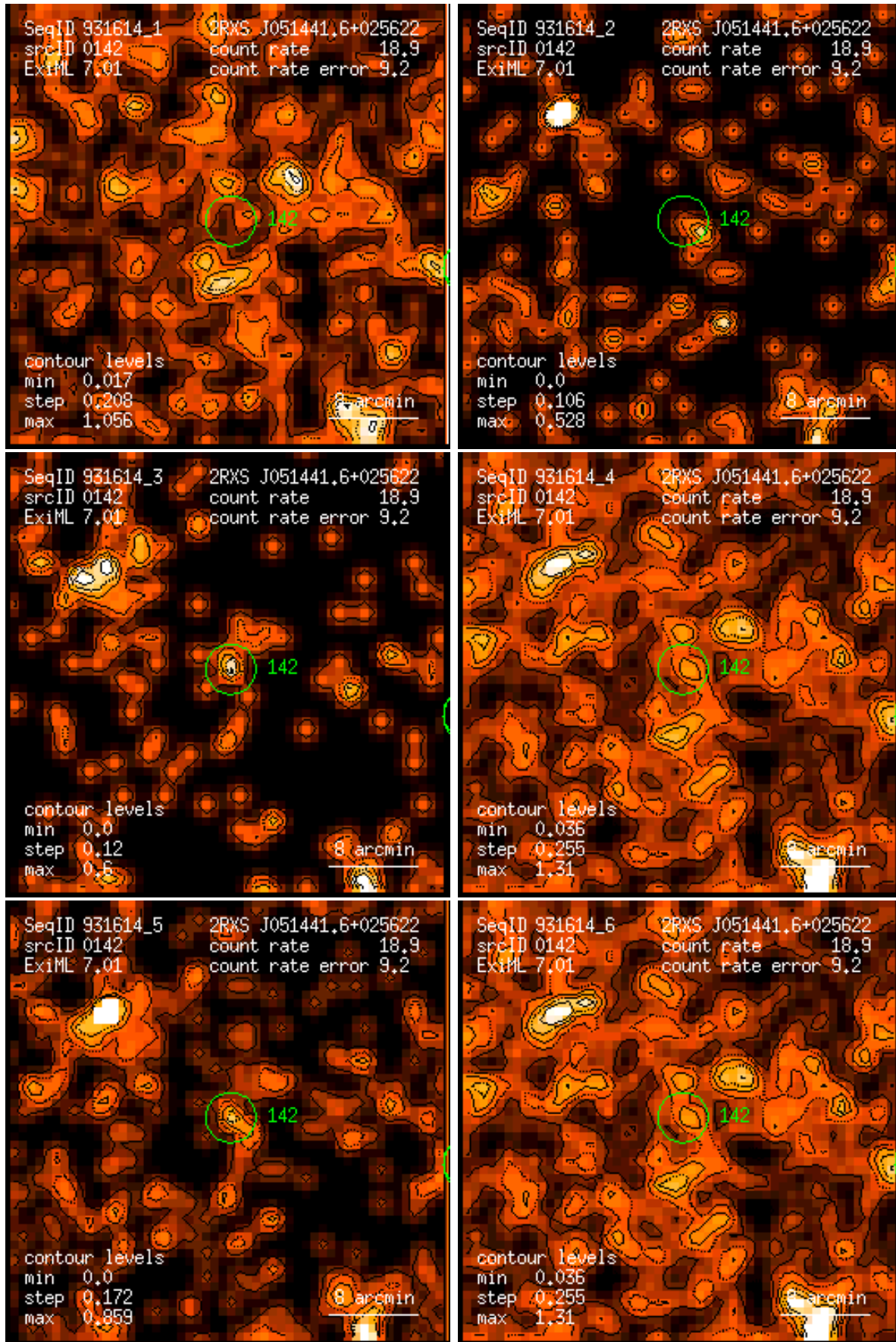
Figure 142: RASS 931614: detection 0142: band rate images, Gaussian filter: (1) PSPC channels 11 – 41, (2) 52 – 90, (3) 91 – 201, (4) 11 – 235, (5) 52 – 201, (6) 11 – 201. Broad band rates in counts/ks. Band rate contour levels in counts/ks/arcmin 2 .
