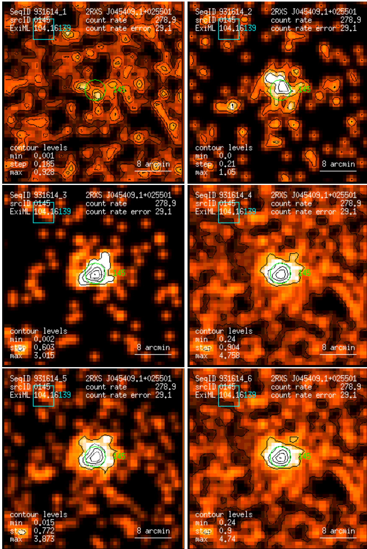
Figure 145: RASS 931614: detection 0145: band rate images, Gaussian filter: (1) PSPC channels 11 – 41, (2) 52 – 90, (3) 91 – 201, (4) 11 – 235, (5) 52 – 201, (6) 11 – 201. Broad band rates in counts/ks. Band rate contour levels in counts/ks/arcmin 2 .
