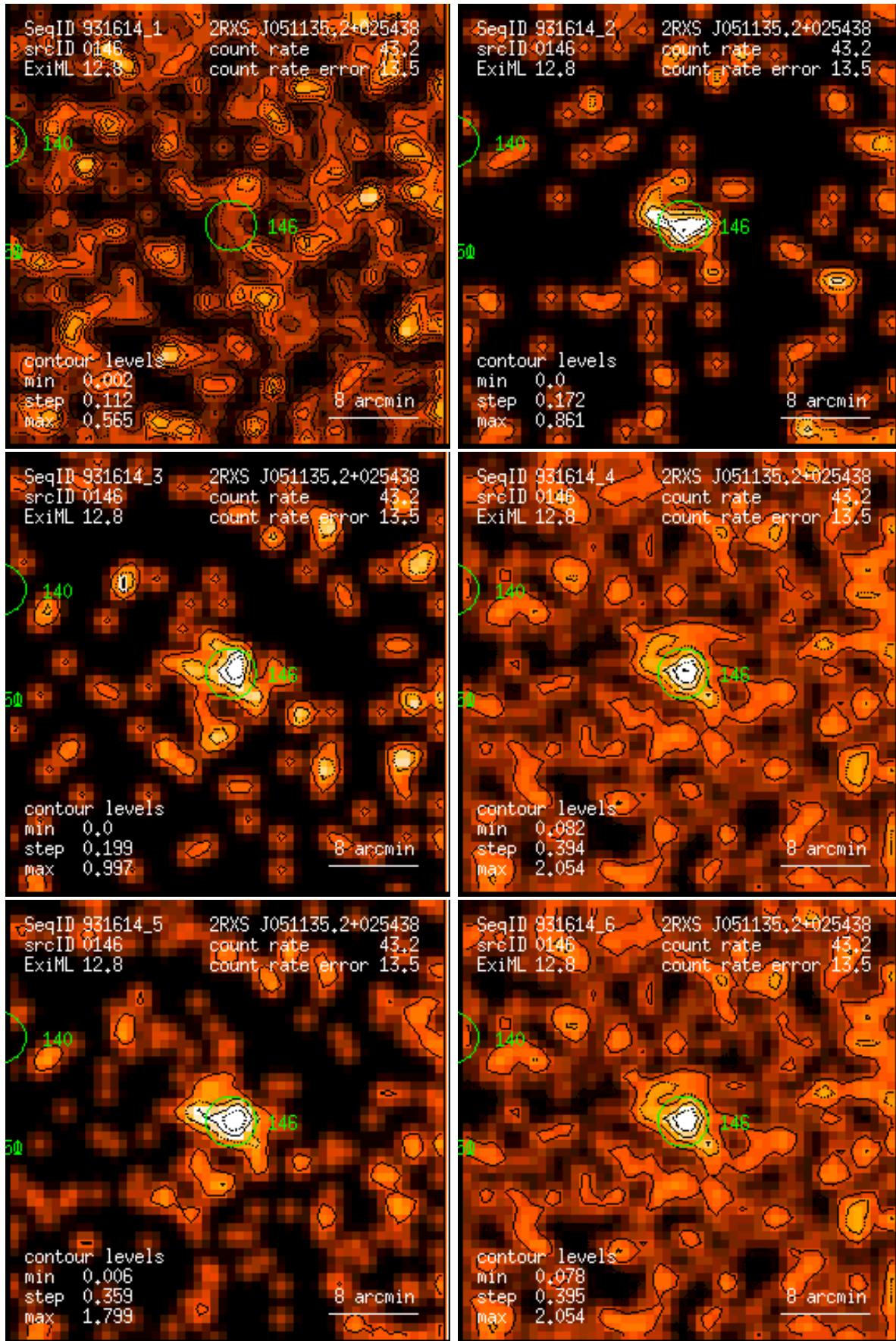
Figure 146: RASS 931614: detection 0146: band rate images, Gaussian filter: (1) PSPC channels 11 – 41, (2) 52 – 90, (3) 91 – 201, (4) 11 – 235, (5) 52 – 201, (6) 11 – 201. Broad band rates in counts/ks. Band rate contour levels in counts/ks/arcmin 2 .
