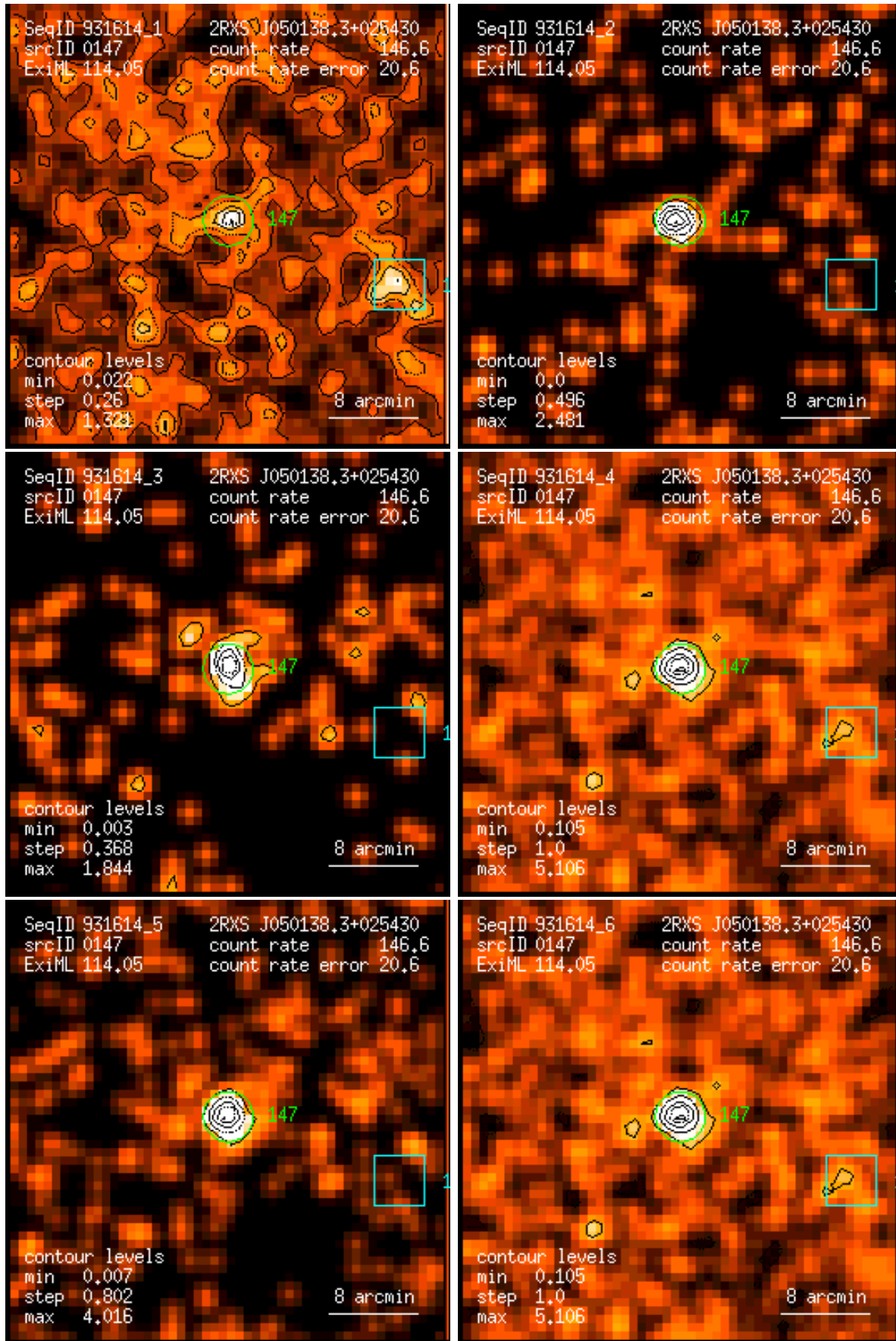
Figure 147: RASS 931614: detection 0147: band rate images, Gaussian filter: (1) PSPC channels 11 – 41, (2) 52 – 90, (3) 91 – 201, (4) 11 – 235, (5) 52 – 201, (6) 11 – 201. Broad band rates in counts/ks. Band rate contour levels in counts/ks/arcmin 2 .
