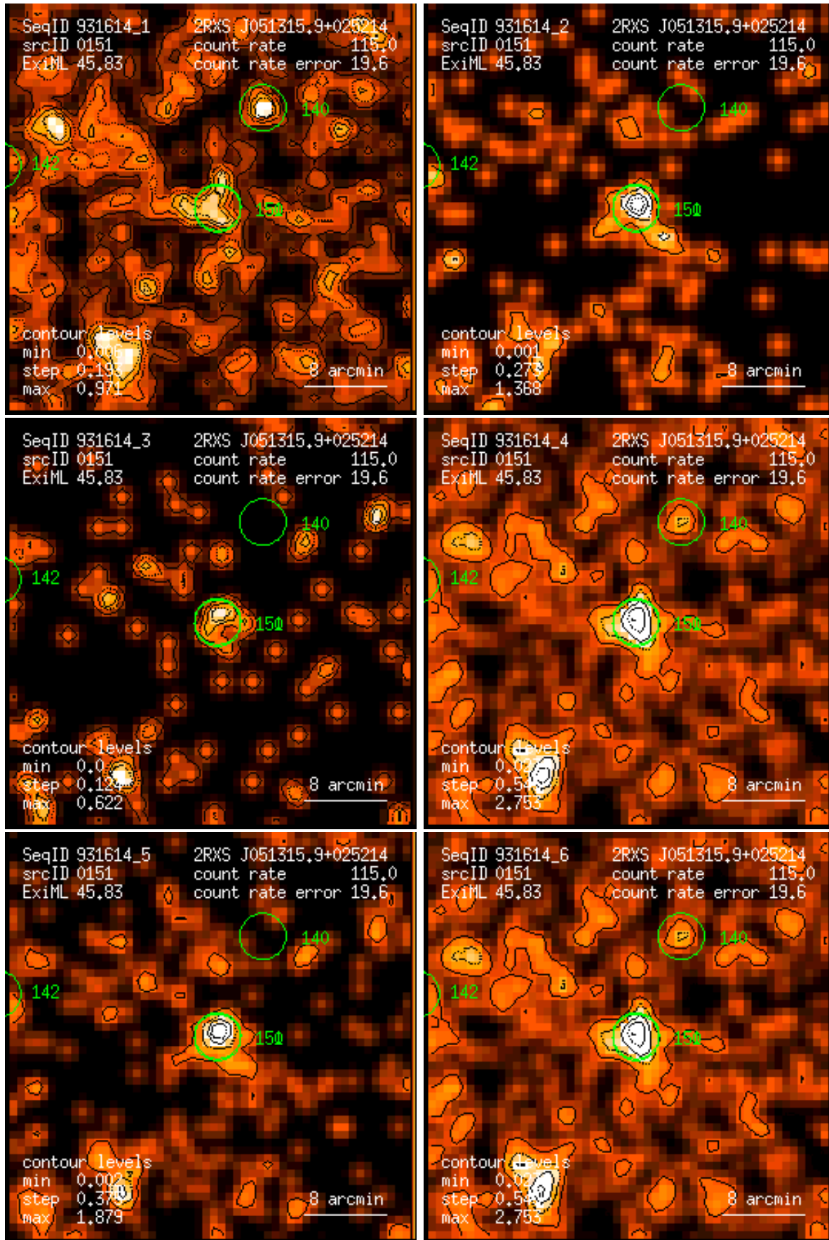
Figure 151: RASS 931614: detection 0151: band rate images, Gaussian filter: (1) PSPC channels 11 – 41, (2) 52 – 90, (3) 91 – 201, (4) 11 – 235, (5) 52 – 201, (6) 11 – 201. Broad band rates in counts/ks. Band rate contour levels in counts/ks/arcmin 2 .
